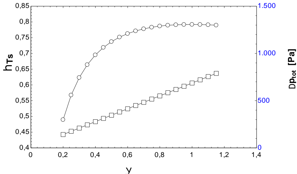
Fig. 6. Effect of load Coefficient \Psi ( DR = 0,7 ; \Phi = 0,3 ): Efficiency and Pressure drop
