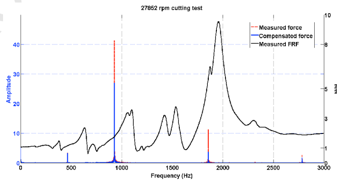
Figure 11: Detailed Frequency domain force signals related to measured transmissibility FRF
