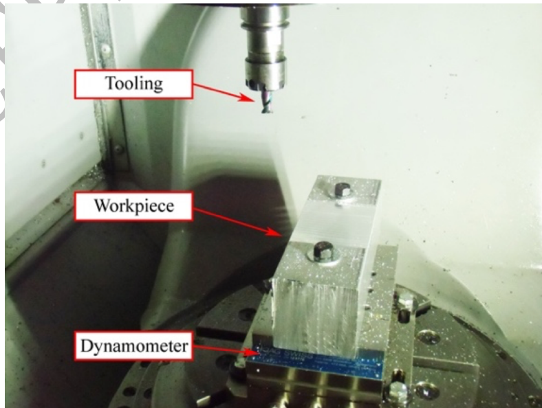
Fig. 3 Test set-up
