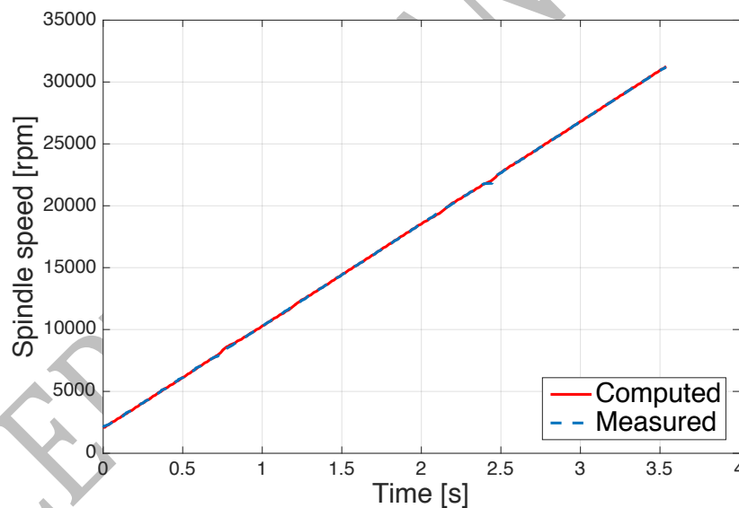
Fig. 8 Spindle speed during SSR computed by proposed method and measured via optical tachometer
