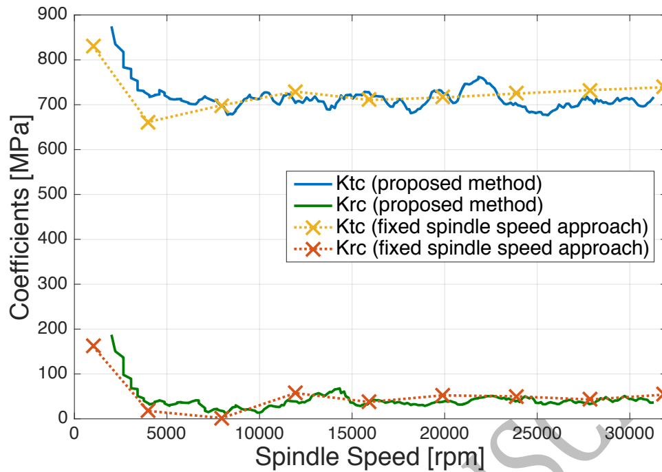
Fig. 12 Coefficients validation compared to fixed spindle speed
