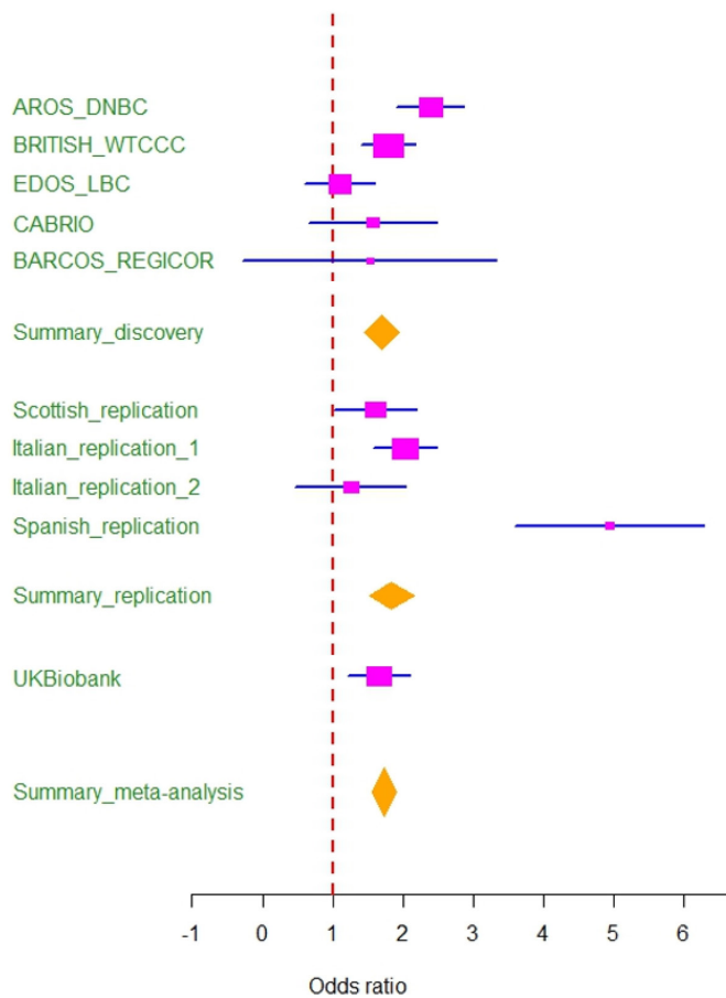
Figure 1 Cohort specific association between rs10190845 and clinical vertebral fracture. The point estimates (squares) and 95% CIs (horizontal lines) for individual studies are shown with the summary indicated by the diamond using a fixed effect model. Summaries are shown for meta-analysis with discovery cohorts only (Summary_discovery), with the first replication cohorts only (Summary_replication), and for the whole three-stage meta-analysis (Summary_meta-analysis). 'BRITISH-WTCCC' shows the results for the combined cohorts CAIFOS, AOGC, DOES and EPIC and the control cohort WTCCC2. 'Scottish replication' corresponds to EDOS-ORCADES cohorts, 'Italian_replication_1' study corresponds to Florence-InCHIANTI cohorts and 'Italian_replication_2' study comprises the Turin and Siena cohorts. Cohort sizes are reflected by square dimensions.
