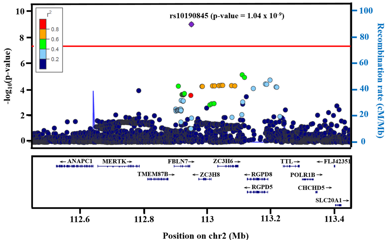
Figure 2 Regional association plots of susceptibility locus for clinical vertebral fracture. The figure shows the results after imputation using 1000G v3 as reference panel. The SNPs are colour coded according to the extent of linkage disequilibrium with the SNP showing the highest association signal from the combined analysis (represented as a purple diamond). The estimated recombination rates (cM/Mb) from HapMap CEU release 22 are shown as light blue lines, and the blue arrows represent known genes in the region. The red line shows the threshold for genome-wide significance ( P=5 \times 10^{-8} ).
