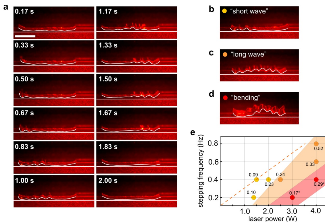
Figure 4 Walking modes of the LCE soft robot. a , Series of photographs showing the deformation wave travelling along the robot body during one stepping cycle. White lines are traced on the photographs along the walking surface and the edge of the robot body for guiding the eye. Scale bar (for all photographs): 5 mm. b , c , d , Different gaits of the soft robot: "short wave", "long wave" and "bending" modes. e , LCE robot modes of locomotion as observed for different laser powers and stepping frequencies. Colored circles correspond to different gaits and the numbers next to each circle are measured average speeds in mm/s. Asterisks mark the conditions where accelerated film damage occurs. Dashed orange line corresponds to a constant laser power per unit area per unit time i.e. laser light intensity/frequency=constant.
