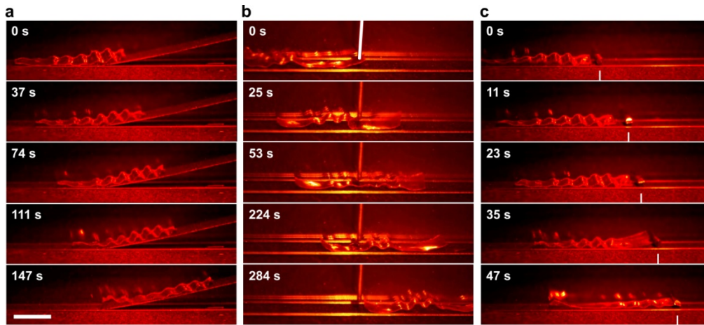
Figure 5 LCE soft robot in various tasks. a , Climbing an 11 degree slope. b , Squeezing through a 0.9 mm high slit. White line is traced in the first photograph along the slit upper wall. c , Moving a metal cylinder with 0.2 mm/s average speed. White tick marks indicate the cylinder center position. Scale bar for all photographs, 5 mm.
