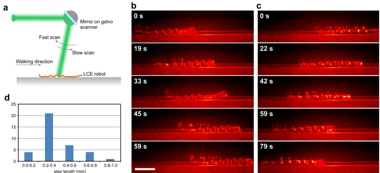
Figure 3 Light driven locomotion of the LCE soft robot. a , Schematic of the experiment. The laser beam is scanned along the robot body with an asymmetric sawtooth signal driving a galvo scanner. Series of photographs for the light driven locomotion in the forward ( b ) and backward ( c ) directions, scale bar for all photographs, 5 mm. d , Histogram of the step lengths for 37 steps taken during the walk in b . Orange filter is used to cut off scattered green light.
