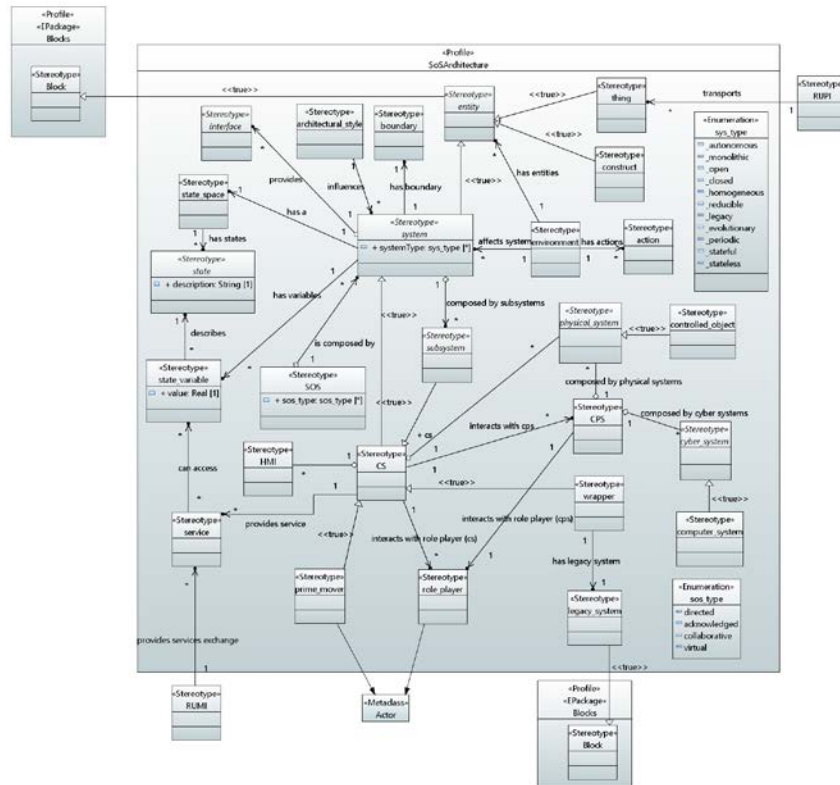
Figure 4-15: SoS Architecture package
