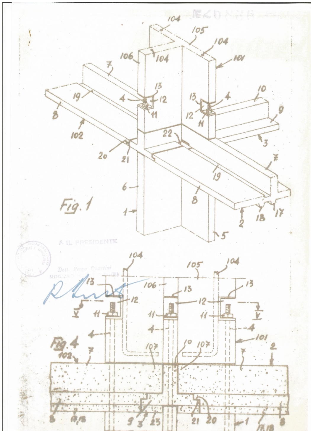
Figure 3: Drawings attached to the patent dossier "Joint system for prefabricated reinforced concrete elements".
