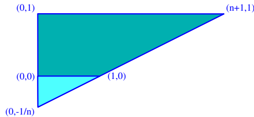
FIGURE 8. Blowing-up \mathbb{C}\mathbb{P}_{(1,n,1)}^2 .
