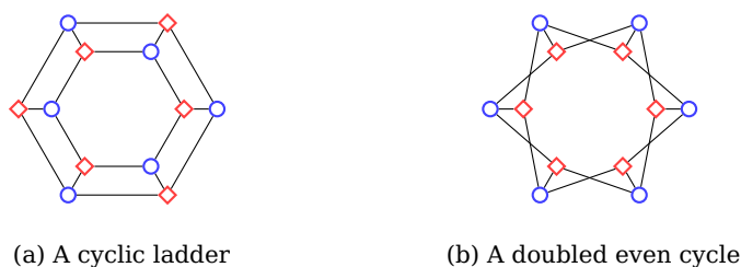
Figure 4: A doubled even cycle is isomorphic to a cyclic ladder.
