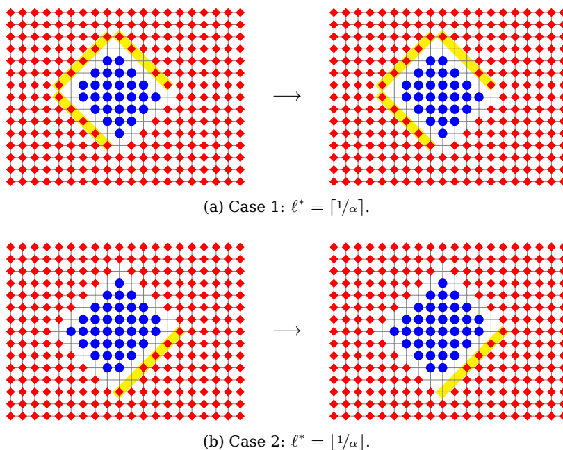
Figure 13: Typical transitions through the critical gate for the doubled torus. The critical length \ell^* in both cases is assumed to be 4. The ‘hole’ can be anywhere in the highlighted region. Once a two-site ‘hole’ is produced, with probability close to 1 a blue particle appears very quickly in the opened-up space.
