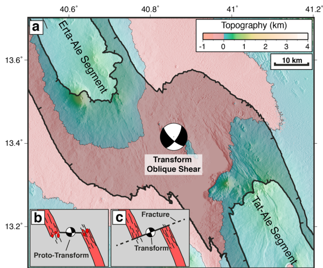
Figure 8. (a) Topography taken from the numerical model at 1.8 Myr (shaded below sea level, light above sea level) overlain on topography from the Giuliatti Plain (pink below sea level) shows good agreement in the location of topographic highs and lows. The oblique, strike-slip faults that are observed in the Giuliatti Plain are caused by the transtensional proto-transform fault, as predicted by the numerical model. Modeling further predicts that the proto-transform fault will rotate in an anticlockwise sense as volcanic segments propagate toward each other (b). The anticlockwise rotation of the proto-transform fault results in the observed rotation of surface faulting in the Giuliatti Plain. The proto-transform fault then develops into a spreading parallel transform fault (c), with pure strike-slip motion. This is then a stable and persistent feature such as transform faults observed at mid-ocean ridges worldwide.
