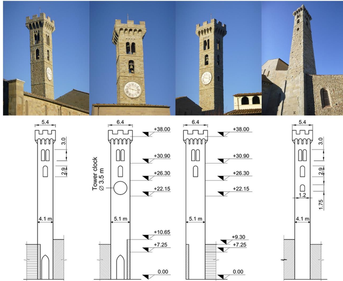
Fig. 1. General and frontal views of Fiesole bell-tower. From left to right: West, South, East and North Faces
