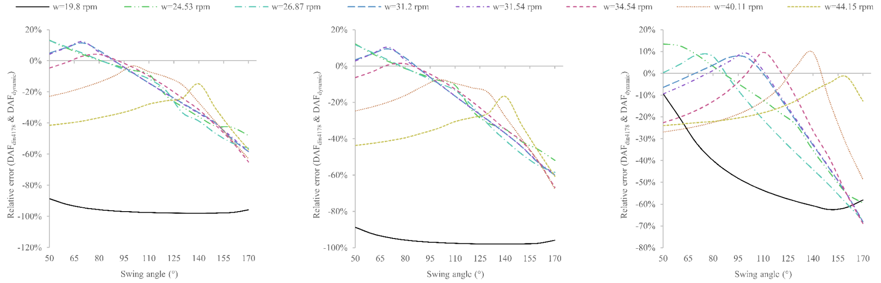
Fig. 13. Relative error of horizontal displacement between DAF_{din4178-2005} & DAF_{dynamics} . Left: 30.9m, E-W; Centre: 26.3m, E-W; Right: 26.3m, N-S.
