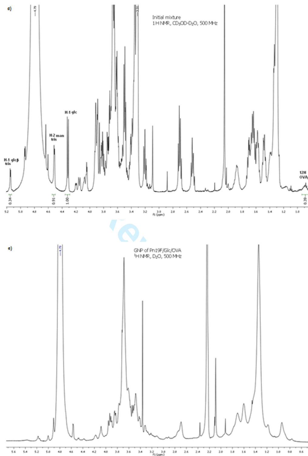
Figure S4 (a) TEM micrographs and (b) histograms of size distribution, (c) UV/Vis adsorption spectrum of gold GNP-2 . (d) ^1\text{H} NMR spectrum (500MHz, \text{CD}_3\text{OD}:\text{D}_2\text{O} 5:1) of the mixture used to prepare GNP and (e) ^1\text{H} NMR spectrum (500MHz, \text{D}_2\text{O} ) of GNP-2 obtained. Integration of selected signals shows that the ratio between trisaccharide 2 , glucose conjugate 4 and OVA \beta is about 45:50:5.
