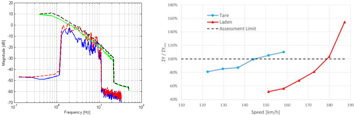
Fig. 14 Left: PSD distribution of lateral (alignment, solid blue) and vertical (longitudinal level, dashed red) for measured defects and the corresponding EN 14363 “High Level” irregularities lateral (solid green) and vertical (dashed black). Right: stability assessment according to EN 14363 in tare and laden conditions for the 4L bogie (from [4]).
