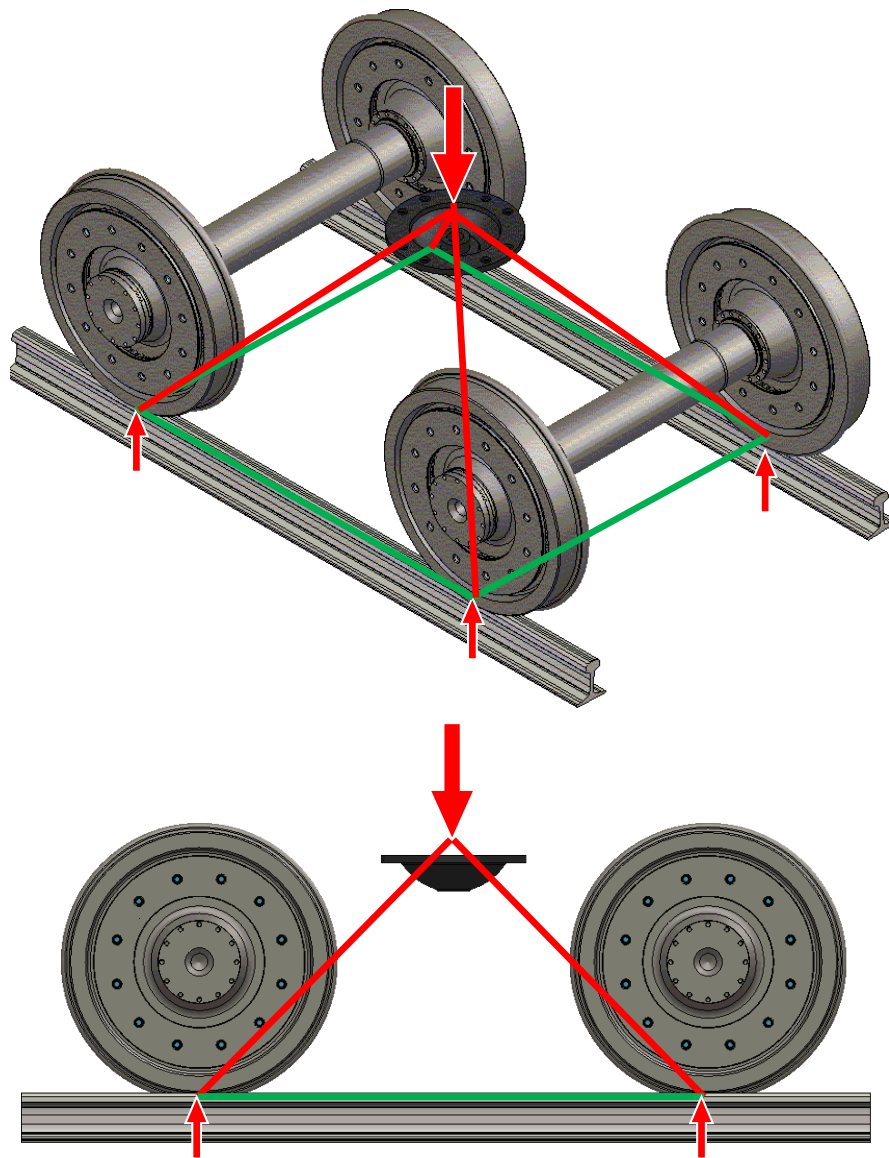
Fig. 4 Sketch of the reactions to the vertical force applied to the centre bowl of a freight wagon.
