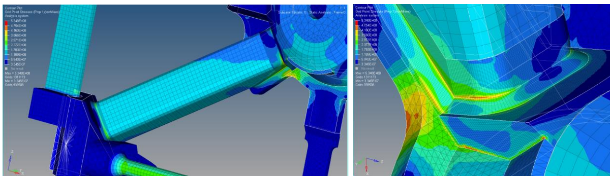
Fig. 10 Validation of the frame of the 4L bogie with the methods described in prEN 17149. Due to the extremely high number of elements, the analysis was applied only locally to weld seams and adjacent areas as specified by the standard.
