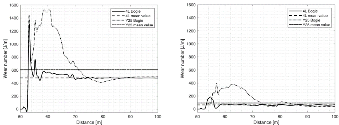
Figure 23. Comparison of wear numbers on the switch blade in the diverging direction for the front wheel (left) and the rear wheel (right) of 4L and Y25 bogies.
