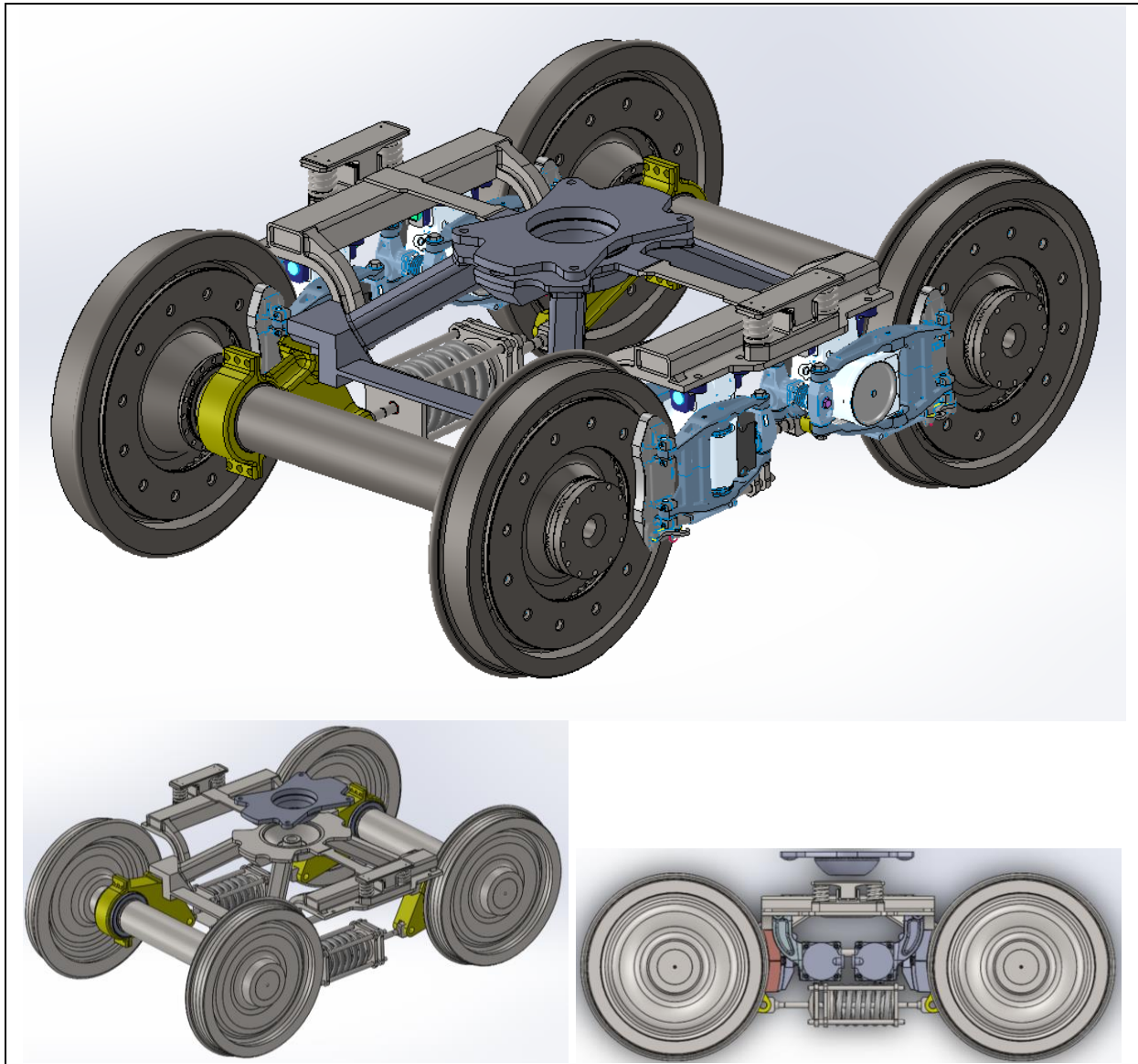
Fig. 6 Top: the 4L bogie with web-mounted brake discs and AIR Wheelsets (mass \cong 4100 kg). Bottom: the 4L bogie with compact brake units acting on thermostable wheels and conventional inboard bearings wheelsets (mass \cong 3700 kg).
