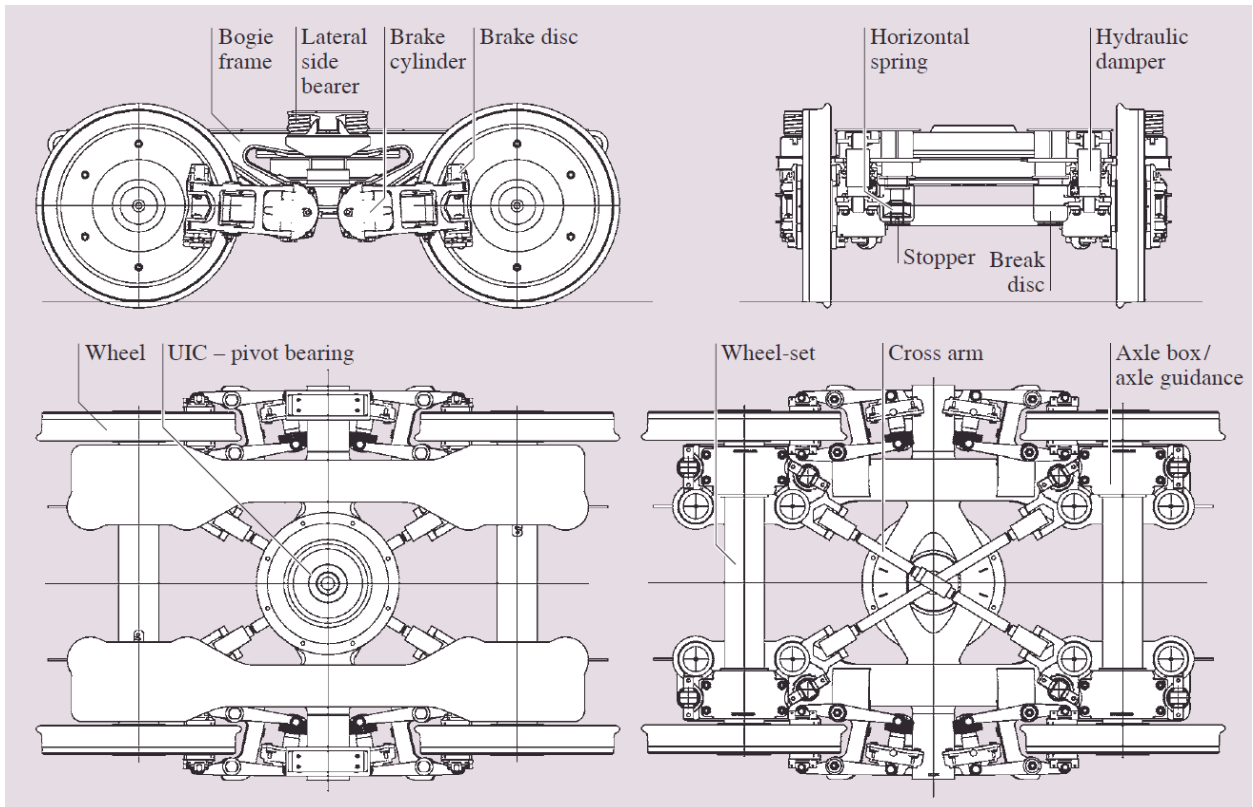
Fig. 3 The Leila bogie, with inboard bearings wheelsets, web-mounted disc brakes, Gigabox primary suspension, two levels of suspension and cross-bracing (lower figure from Grote Antonsson - Springer Handbook of Mechanical Engineering, ch. 13.3 Railway Systems – Railway Engineering)
