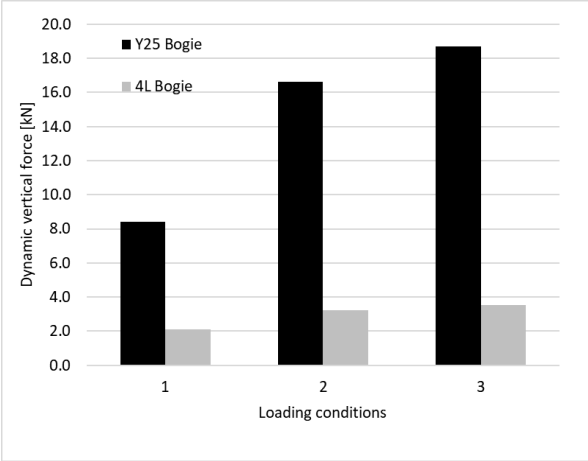
Figure 22. Vertical dynamic peak force in empty condition (1), partially laden condition (2), fully laden condition (3). Speed = 80 km/h in the through direction.
