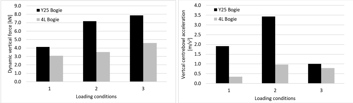
Figure 20. Dynamic vertical force (left) and vertical centre bowl acceleration (right) in empty condition (1), partially laden condition (2), fully laden condition (3).
