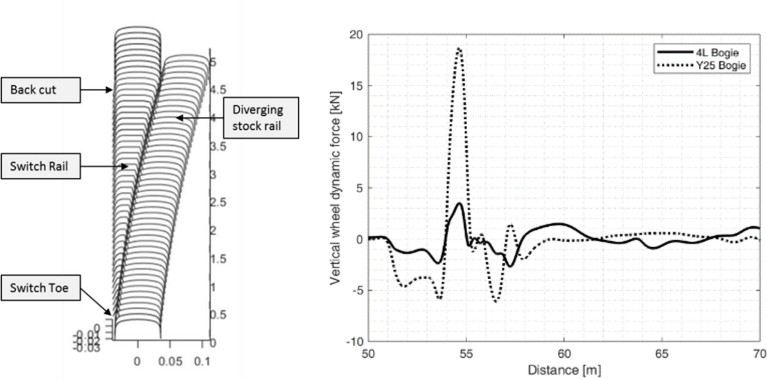
Figure 21. Comparison of the vertical dynamic forces in the laden case at 80 km/h in the through direction.
