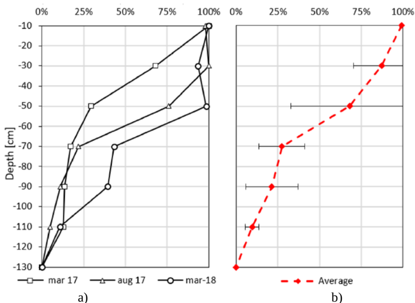
Fig. 2. \text{CH}_4 oxidation efficiency of BW8: a) of each monitoring campaign b) average of the three monitoring campaigns
