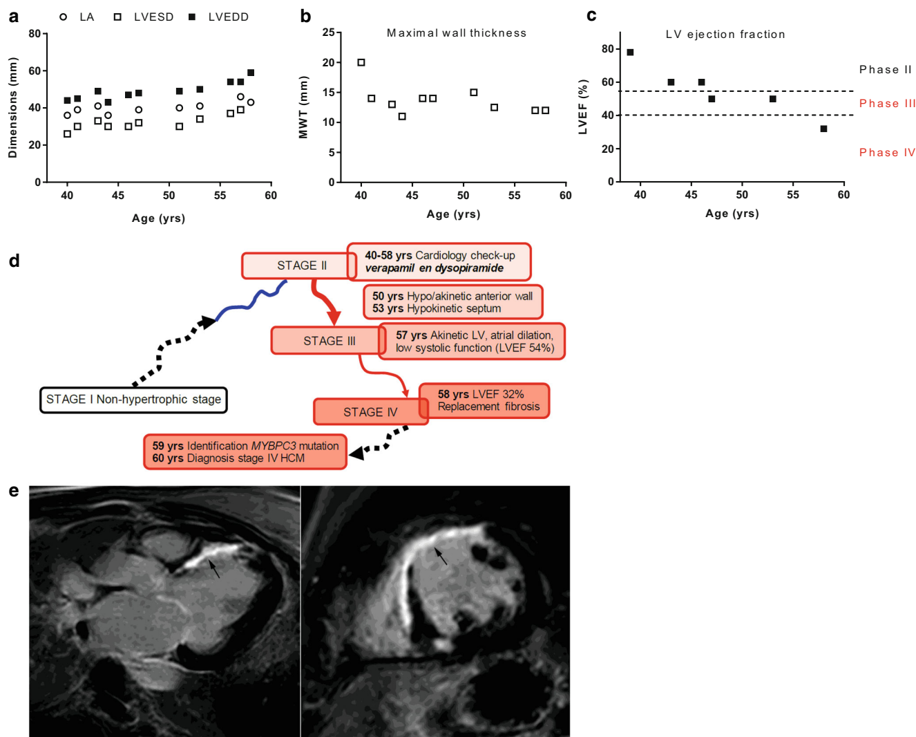
Fig. 4 Progression of disease in patient case 1. a Progressive increase in cardiac dimensions ( LA Left atrium, LVESD and LVEDD Left ventricular end-systolic and end-diastolic dimensions), b decline in maximal wall thickness (MWT) and c a decline in LV ejection fraction (LVEF). d The different disease stages of the patient. e Cardio magnetic imaging at stage IV of the disease showing a dilated heart and extensive late gadolinium enhancement ( arrow )
