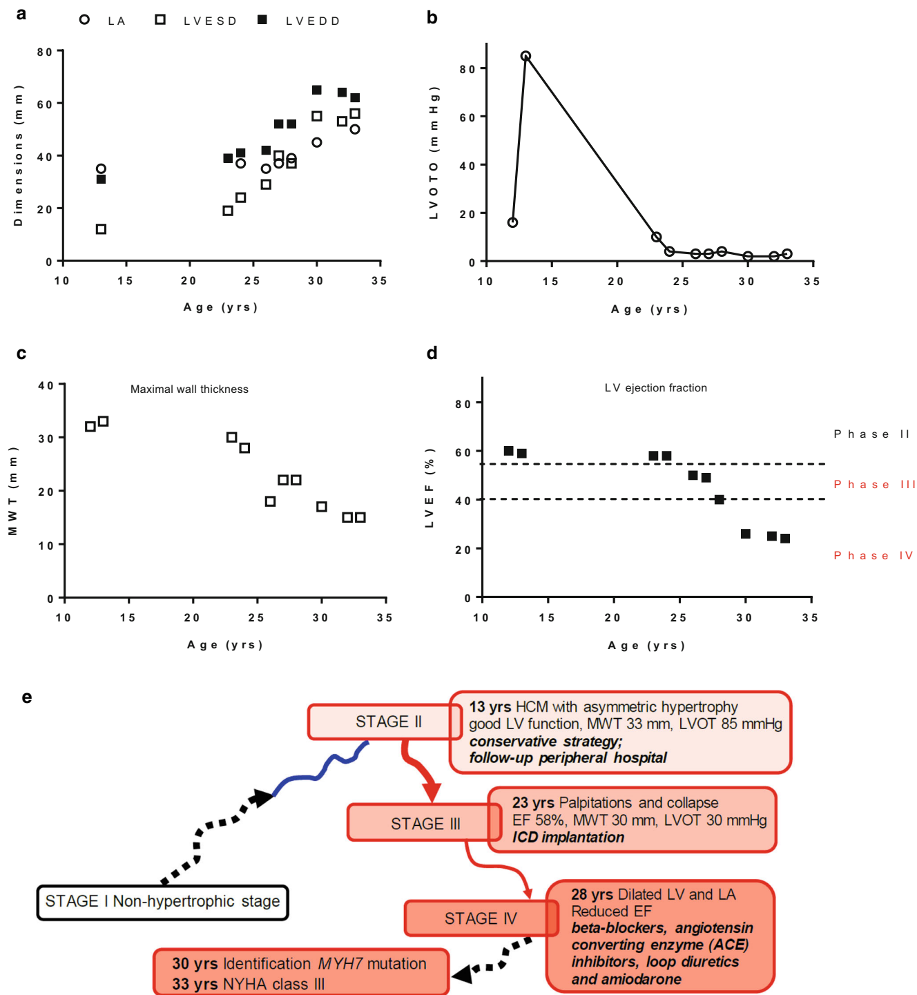
Fig. 2 Progression of disease in patient case 1. a Progressive increase in cardiac dimensions, b a rise and subsequent decline in LVOTO, c a gradual decrease in MWT and d LV ejection fraction, e the different disease stages of the patient (LA Left atrium, LVESD Left ventricular end-systolic dimensions, LVEDD Left ventricular end-diastolic dimensions, LVOTO LV outflow tract obstruction, MWT Maximal wall thickness, LVEF LV ejection fraction [LVEF])
