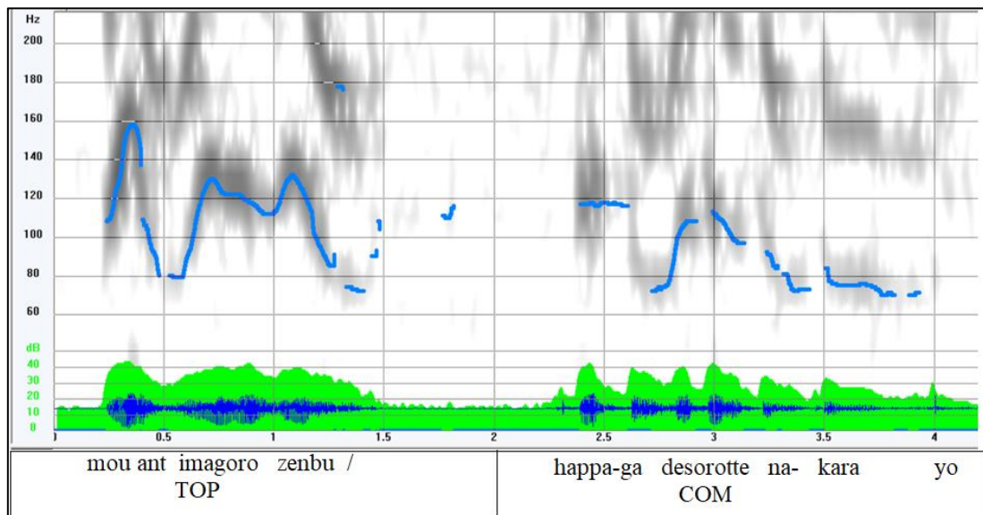
Figure 4: F0 track of example 3.
