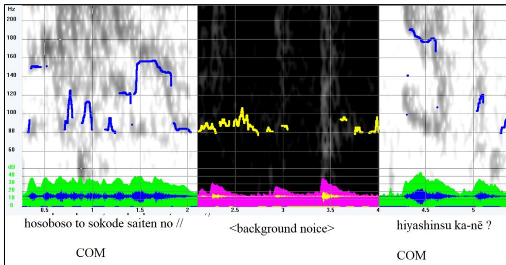
Figure 2: F0 track of example 1. 8
