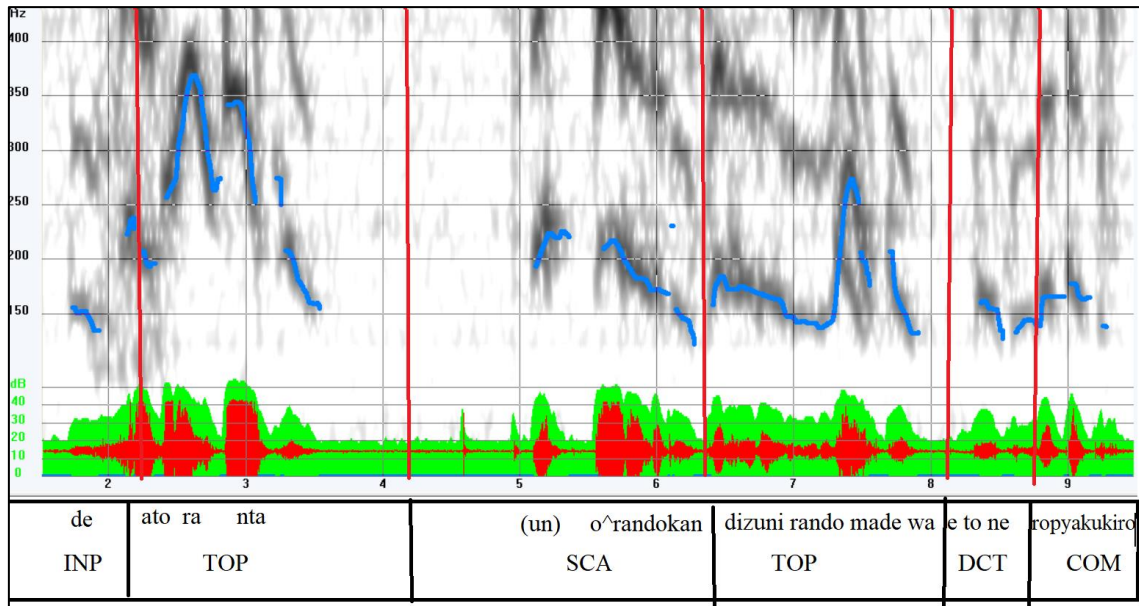
Figure 9: F0 track of example 8.
