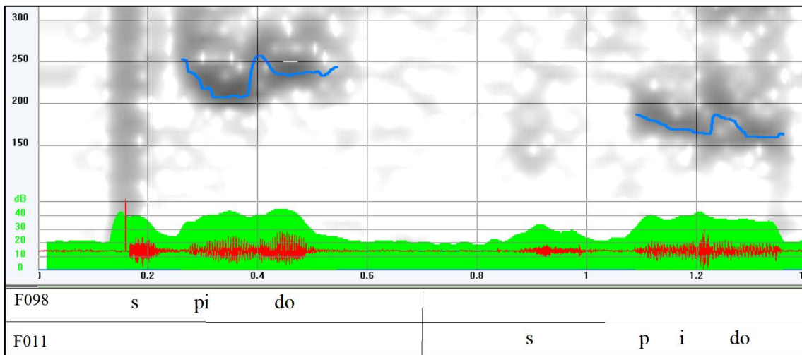
Figure 5: F0 track of example 4.
