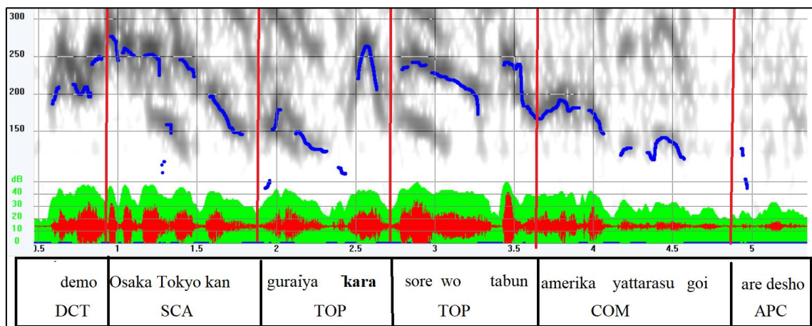
Figure 10: F0 track for the first formant in example 9.
