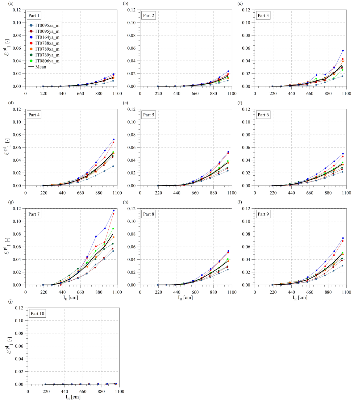
Figure B.17: The IDA curve sets and corresponding mean curves for the ten (10) parts of the Brick House: plots of first principal plastic strain ( \varepsilon_1^{pl} ) versus I_H (a-j).
