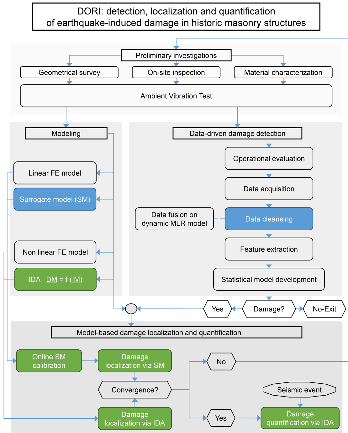
Figure 1.1: General framework of the DORI methodology: D amage identification based on O perational modal analysis & R apid surrogate modeling & I ncremental dynamic analysis.
