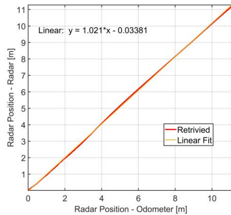
Fig. 22. Comparison between radar and odometer wheel, using a fence wall as reference for the radar
