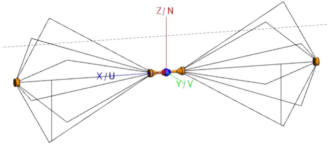
Fig. 2. CAD model of the biconical antenna.
