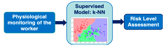
Fig. 7. Block scheme of the proposed classification system.
