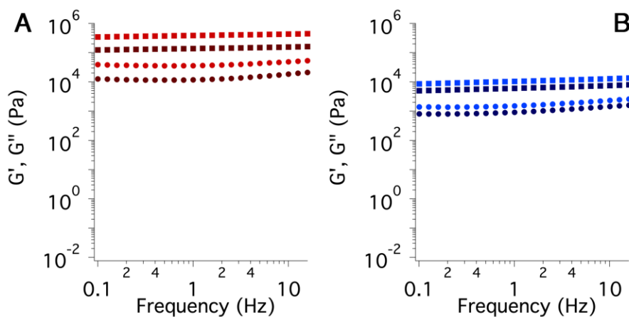
Figure 3. Frequency sweep measurements of systems with GC and alkaline nanoparticles - G' (■), G'' (●). Error bars are included in the dimensions of the markers. Measurements were repeated at least twice on duplicate samples. (A) GC-OH3 after 1 day and 7 days from the preparation (dark red and light red markers, respectively). (B) GC-CO3 after 1 day and 7 days from the preparation (dark blue and light blue markers, respectively).
