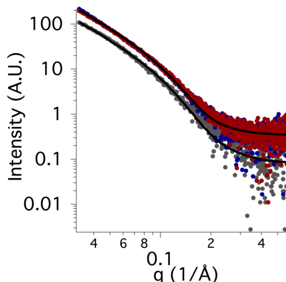
Figure 5. SAXS curves of the three selected samples: GC, gray circles; GC-OH3, red circles; GC-CO3, blue circles. Fitting lines are represented as continuous black curves.
