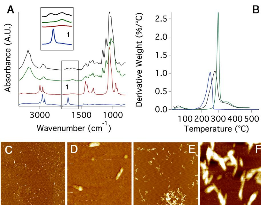
Figure 1. (A) ATR-FTIR spectrum of oleic acid (blue), DMSO (red), CNC (green) and GC (black). (B) DTG curves of oleic acid (blue), CNC (green) and GC (black). (C-D) AFM pictures of CNC over a freshly cleaved mica sheet (10 x 10 \mu\text{m}^2 and 1 x 1 \mu\text{m}^2 , respectively). (E-F) AFM picture of GC over a freshly cleaved mica sheet (10 x 10 \mu\text{m}^2 and 1 x 1 \mu\text{m}^2 , respectively).
