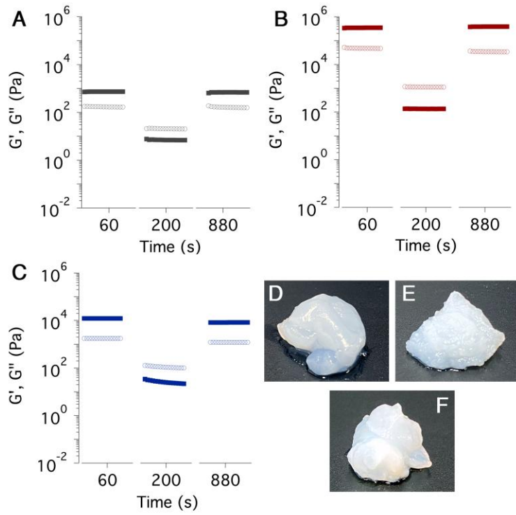
Figure 4. Top row (right and left panels) and bottom row (left panel): three interval thixotropy tests (3ITT) of GC (A), GC-OH3 (B) and GC-CO3 (C) - G' (■), G'' (○). Bottom row, right panel: visual aspect of the samples: GC (D), GC-OH3 (E) and GC-CO3 (F). Error bars are included in the dimensions of the markers. Measurements were repeated at least twice on duplicate samples.
