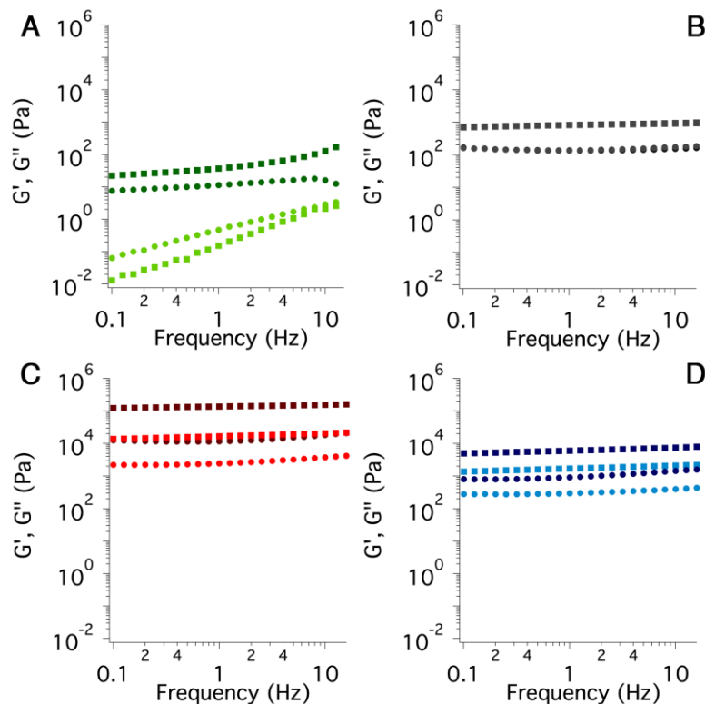
Figure 2. Frequency sweep measurements of systems with CNC and GC - G' (■), G'' (●). Error bars are included in the dimensions of the markers. Measurements were repeated at least twice
