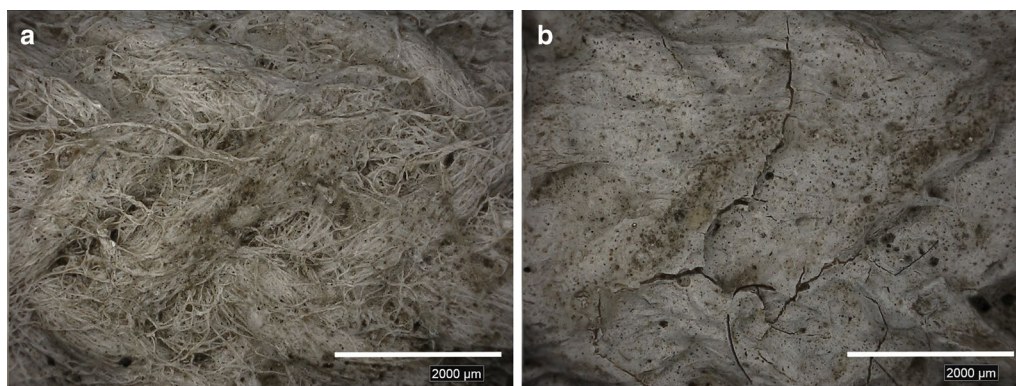
Fig. 4 High-resolution digital (HIROX) images of a rope showing details such as thin paint layers, visible fibres ( a ), cracks in the coating/paint layers ( b ), general yellowing of the surface and embedded soil. The scale bar is 2 mm, and the magnification 50×. Photo Tate 2017, © The estate of Eva Hesse, courtesy Hauser & Wirth, Zürich
