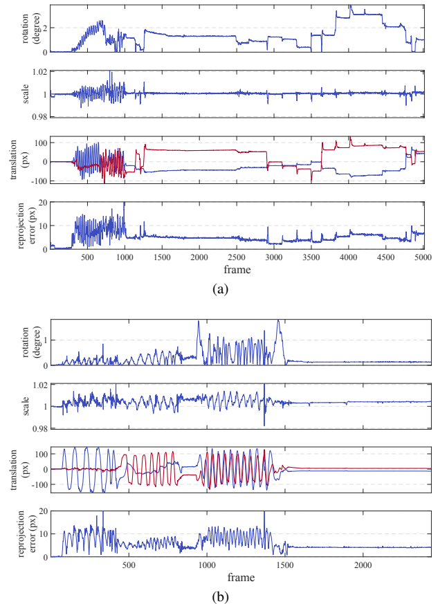
Fig. 5: Decomposition of EIS frame transformation according to a similarity for (a) Huawei P9 Lite and (b) Xiaomi M2 A1 videos. x and y translation components are indicated respectively in blue and red (best viewed in color and zoomed in).
