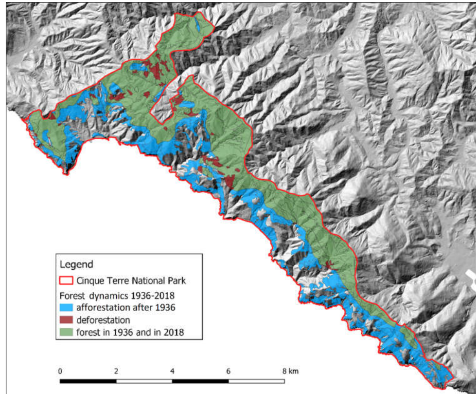
Figure 2. Overlapping the forest maps of 1936 and 2018 allowed identification of the new forest surfaces (blue), the deforested areas (red) and the areas that are currently covered by forests and that were already forests in 1936 (green).
