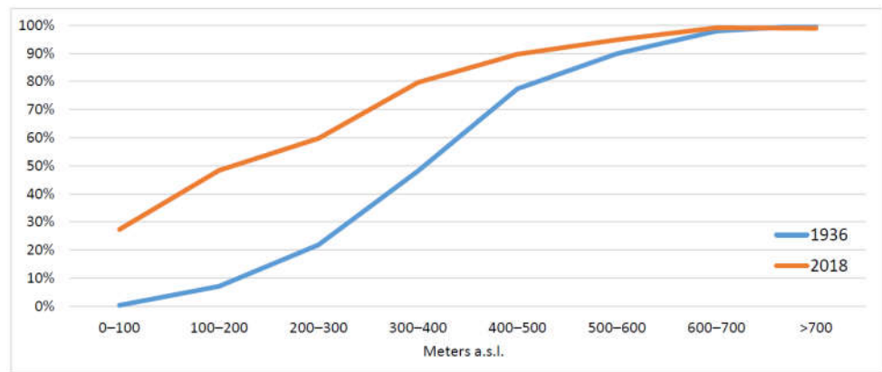
Figure 3. Percentages of the total surface of the Cinque Terre National Park occupied by forests in 1936 and in 2018 according to different altitudinal ranges.
