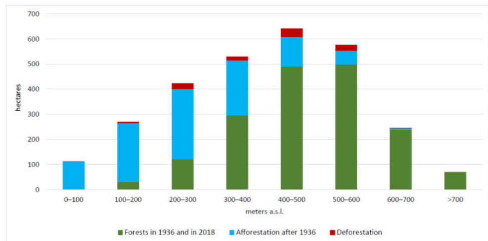
Figure 4. Forest transformations in the period 1936–2018 according to the altitudinal ranges.
