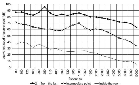
FIGURE 2: Sound spectra measured at various distances from the fan, inside the duct: second case study. ( L_{eq} = 40 dBA in the receiving room).
