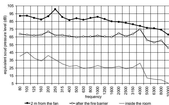
FIGURE 1: Sound spectra measured at various distances from the fan, inside the duct: first case study. ( L_{eq} = 39 dBA in the receiving room).
