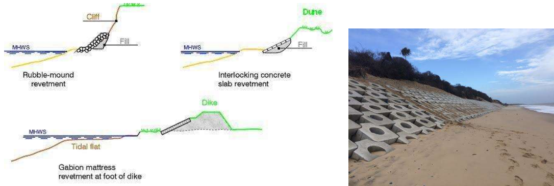
Figure 2–36 (A) Revetments types, image source: www.marinespecies.org ; (B) Concrete block revetment at Dawlish (UK), imagine source: www.networkrailmediacentre.co.uk .
