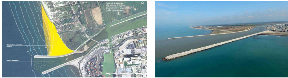
Figure 2-33 Armored river mouth at Arno River in Tuscany (Central Tyrrhenian coast of Italy); (A) design of the structure, image source: www.autoritaportualeregionale.toscana.it ; (B) Armoring after its completion, image source Ing. Paolo Ghezzi.
