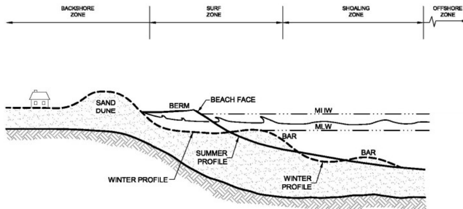
Figure 2-12 Summer and Winter profiles of a typical Pacific Coast, modified from Bascom, 1964. Image source www.fema.gov .
