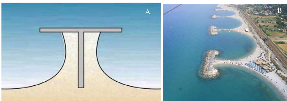
Figure 2-31 (A) Simplified design of a basic composite groin (Paganelli et al., 2014); (B) Composite groins field at Paola, South of Italy, where they were realized to protect the railway limiting the coastal zone visible just on the backshore; image source: www.confesercenticosenza.it
