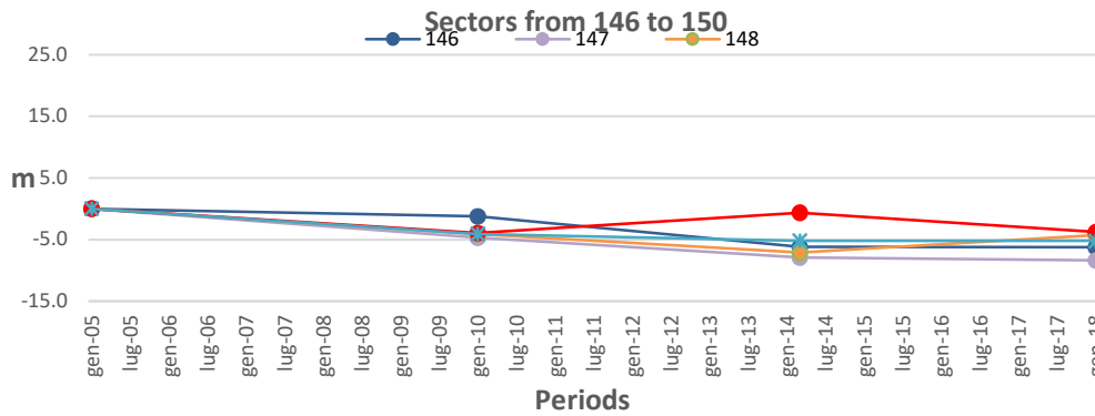
Figure 5-13. Shoreline displacement within the sectors from 146 to 150 (sub-unit C) in the period 2005-2018.
