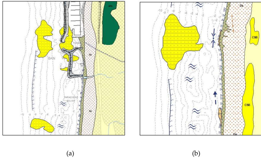
Figure 6-3 Calcareniti sabbiose del Biserno CSB (late Pleistocene) are represented as yellow deposits; (a) at the harbor are (b) at La Punticella location. See geological legend in figure 6.2.
