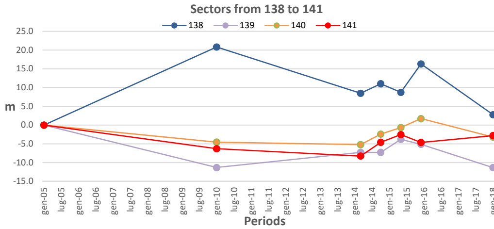
Figure 5-11. Shoreline displacement within the sectors from 138 to 141 (sub-unit B) in the period 2005-2018
