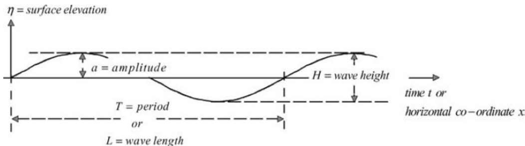
Figure 2-14 Sine wave from Holthuijsen, 2007.
