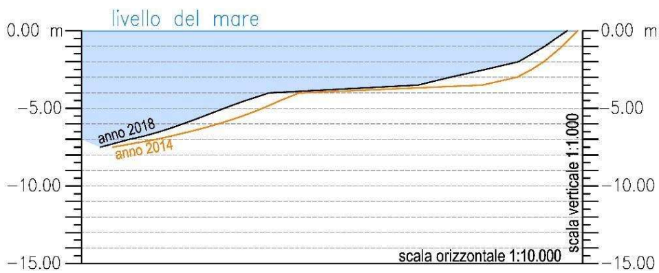
Figure 5-47. CAD cross-section at sector 168. It was drawn on the bathymetric maps after the field surveys done in 2014 and 2018.
