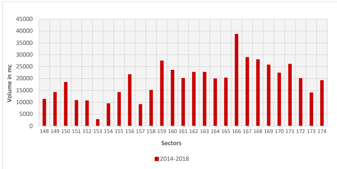
Figure 5-25. Volumetric variations between “-1m” and “-7m” depth in the period 2014-2018 (May) at the Southern part of the San Vincenzo’s Unit -sub-units B and C- (Bianco et al., 2020).
