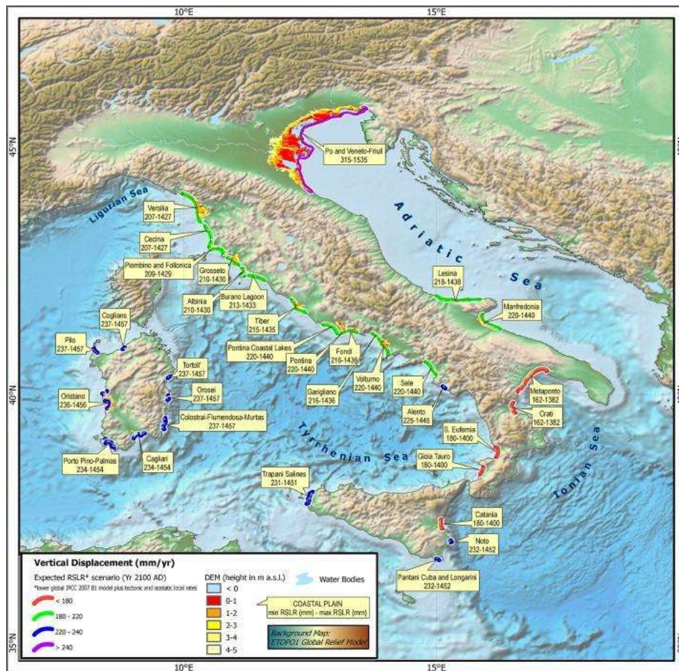
Figure 2-2 Vulnerable areas to coastal inundation due to SLR projection at 2100 (Lambeck et al., 2011).
