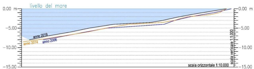
Figure 5-31. CAD cross-section at sector 133. It was drawn on the bathymetric maps after the field surveys done in 2006, 2014 and 2018.
