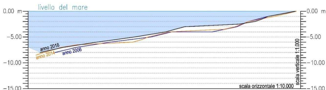
Figure 5-42. CAD cross-section at sector 142. It was drawn on the bathymetric maps after the field surveys done in 2006, 2014 and 2018.
