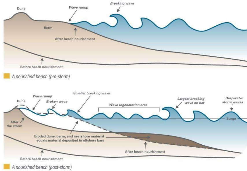
Figure 2-38 Simplified expected effect of an artificial nourishment in respect to waves. Image source: US Army Corps of Engineers www.nad.usace.army .
