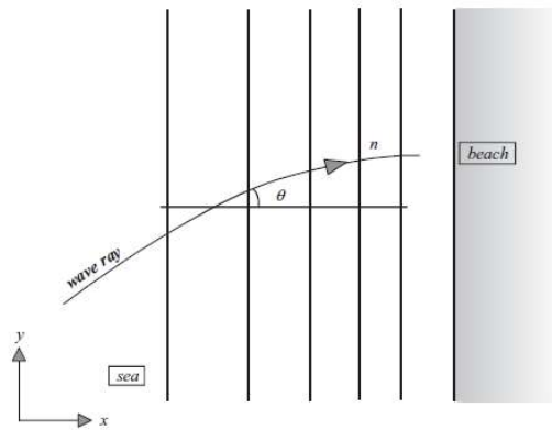
Figure 2–15 Schematic representation of Snell's law, and ideal representation of the angle \theta , from Holthuijsen, 2007.
