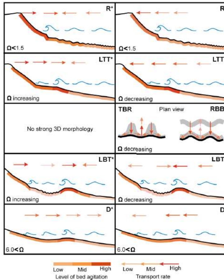
Figure 2–20 Beach state model from Aagaard et al., 2013; \Omega is the Surf-Scaling Parameter, while sediment stirring and net sediment transport are respectively explained by the color intensity bar, and the color intensity arrows. The states are representative of Reflective ones ( R, R^* ), Dissipative ( D, D^* ) and Intermediate low-tide terrace ( LTT and LTT^* ), transverse-bar and rip ( TBR ), rhythmic-bar and beach ( RBB ), longshore-bar and through ( LBT and LBT^* ).
