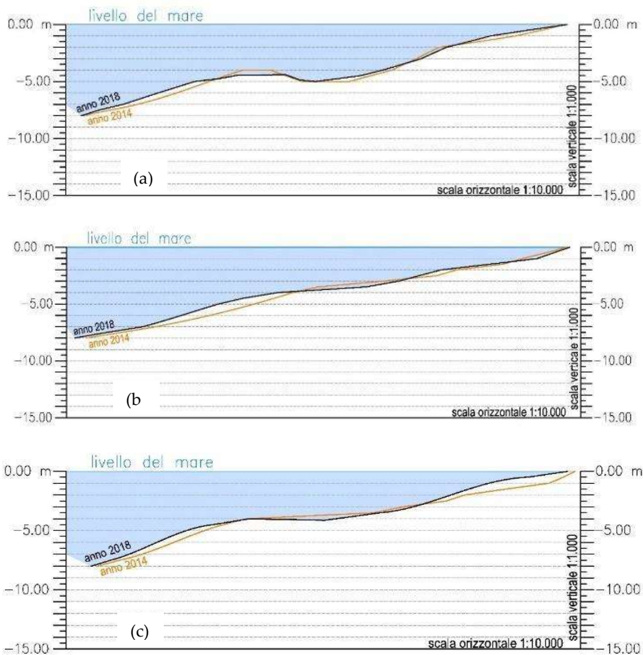
Figure 5-45. (a) CAD cross-section at sector 150 (b) CAD cross-section at sector 153; (c) CAD cross-section at sector 157. They were drawn on the bathymetric maps after the field surveys done in 2014 and 2018.
