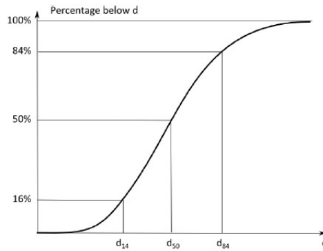
Figure 2-9 Log-normal distribution of sediment sizes (Mangor et al., 2017).
