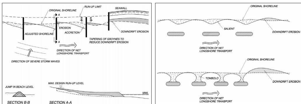
Figure 2-25 Hard structures functioning (A) Typical beach configuration with groins; (B) Typical beach configurations with detached nearshore breakwaters (images source: www.gfdrr.org/en ).
