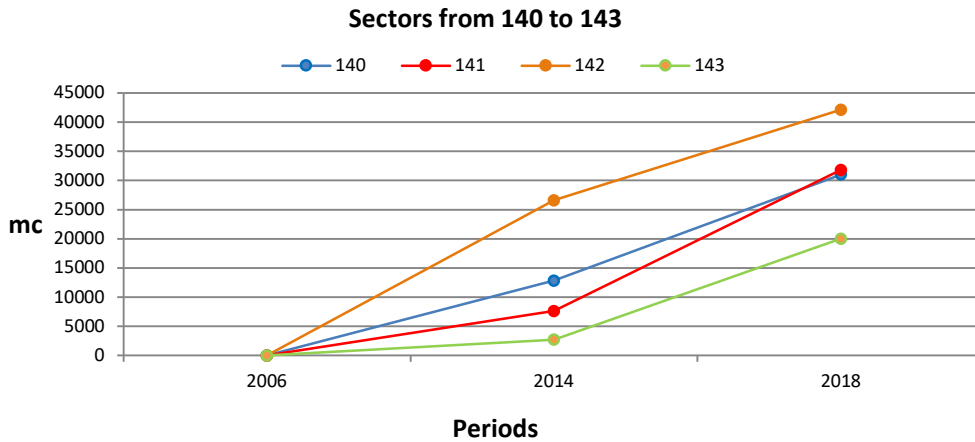
Figure 5-23. Volumetric variations between the isobaths “1m” and “7m”, for sectors from 140 to 143 in the period 2006-2018.
