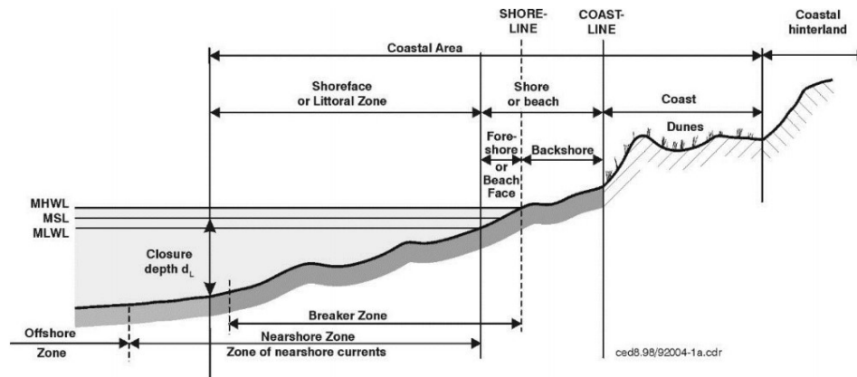
Figure 2-8. Ideal zonation of the coastal zone, after Shore Protection Manual (Coastal Engineering Research Center, 1984). MLWL= Mean Low Water Level; MSL= Mean Sea Level, MHWL= Mean High-Water Level
