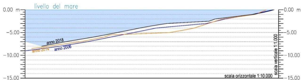
Figure 5-30. CAD cross-section at sector 132. It was drawn on the bathymetric maps after the field surveys done in 2006, 2014 and 2018.
