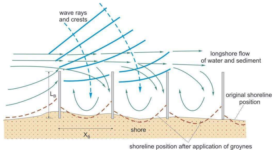
Figure 2-27 Interaction of Groins, waves, currents, and shore; image source: www.marinespecies.org .
