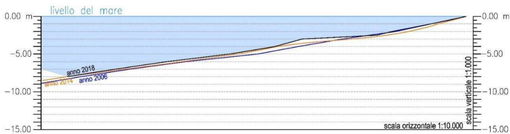
Figure 5-38. CAD cross-section at sector 140. It was drawn on the bathymetric maps after the field surveys done in 2006, 2014 and 2018.
