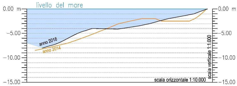
Figure 5-46. CAD cross-section at sector 162. It was drawn on the bathymetric maps after the field surveys done in 2014 and 2018.
