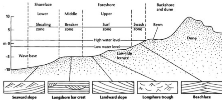
Figure 2-21 Schematic beach's profile showing the main components of the seaward facing barrier island (Prothero, 1990).
