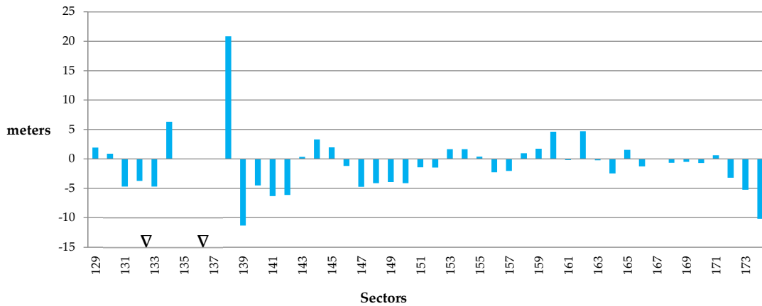
Figure 5-1. Shoreline displacement at San Vincenzo test site in the timeframes 2005-2010.
