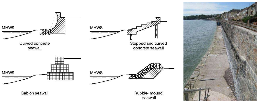
Figure 2–37 (A) Seawall types , image source: www.marinespecies.org (B) Seawall protecting railway at Dawlish (UK), imagine source: www.networkrailmediacentre.co.uk .
