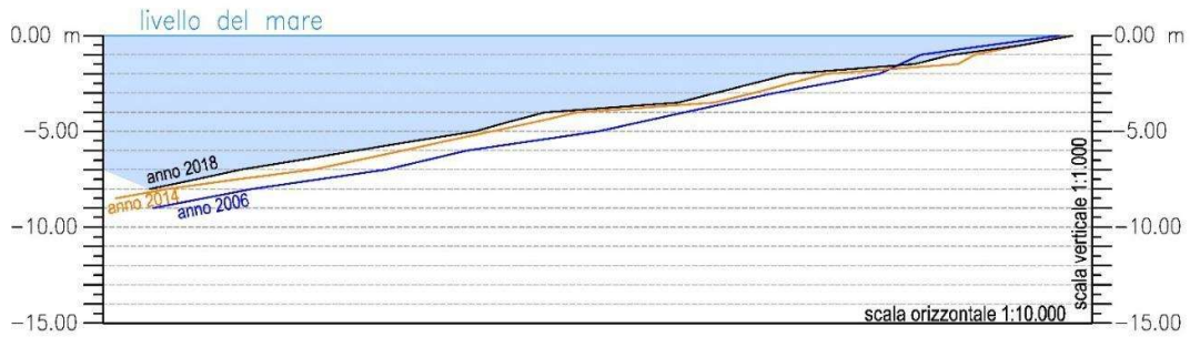
Figure 5-44. CAD cross-section at sector 147. It was drawn on the bathymetric maps after the field surveys done in 2006, 2014 and 2018.
