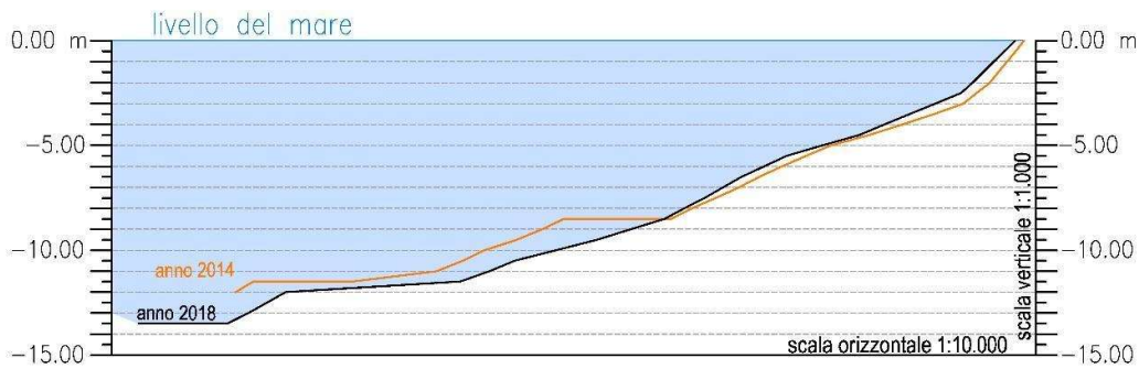
Figure 5-49. CAD cross-section at sector 173. It was drawn on the bathymetric maps after the field surveys done in 2014 and 2018.
