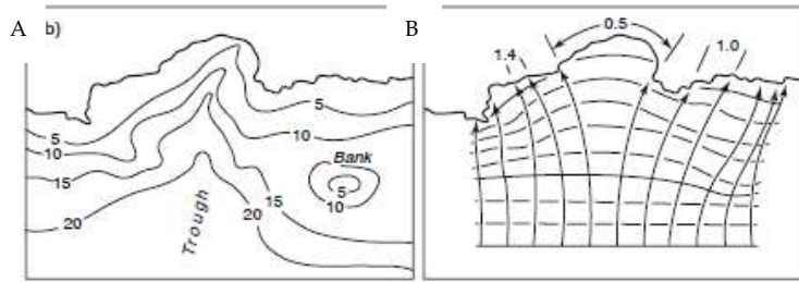
Figure 2-17 Refraction of waves over a through, modified from Bird, 2008; (A) isobaths show different slopes and evolution; (B) energy distribution during refraction, where the numbers indicate the refraction index.
