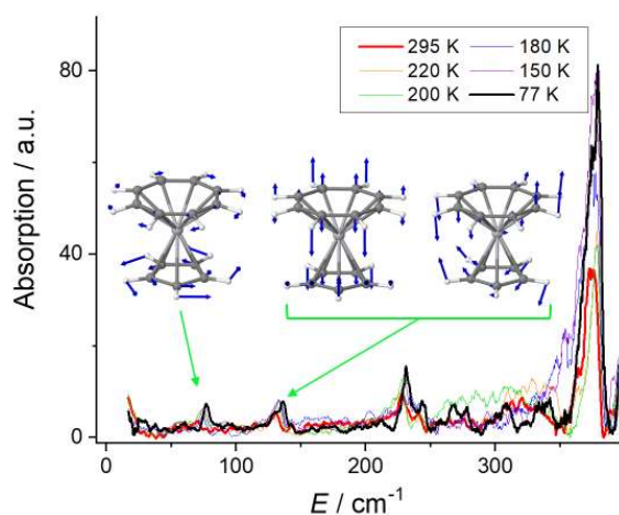
Figure 4. Absorption of THz radiation of 1 dispersed in high-density polyethylene at different temperatures. In the inset, the displacements vectors computed for the first three lowest-energy vibration modes are reported and here tentatively assigned to the observed IR bands.
