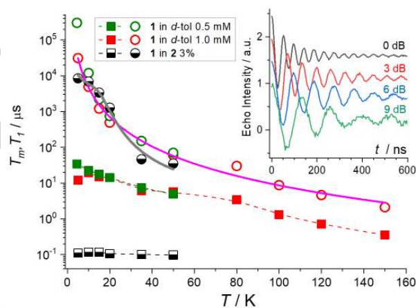
Figure 3. Temperature dependence of T_1 and T_m extracted from Q-band pulsed-EPR experiments performed for deuterated toluene frozen solutions of 1 at two concentrations, and for a solid solution of 1 in 2 . The solid lines represent the best-fit curves reproducing T_1 (see text). Broken lines are only a guide to the eye. The inset presents the normalized echo intensity in nutation experiments for the 0.5 mmol \text{L}^{-1} solution of 1 at T=80 K.
