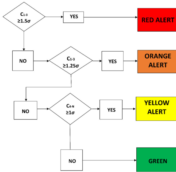
Figure 6. Decisional algorithm used for calibration.
