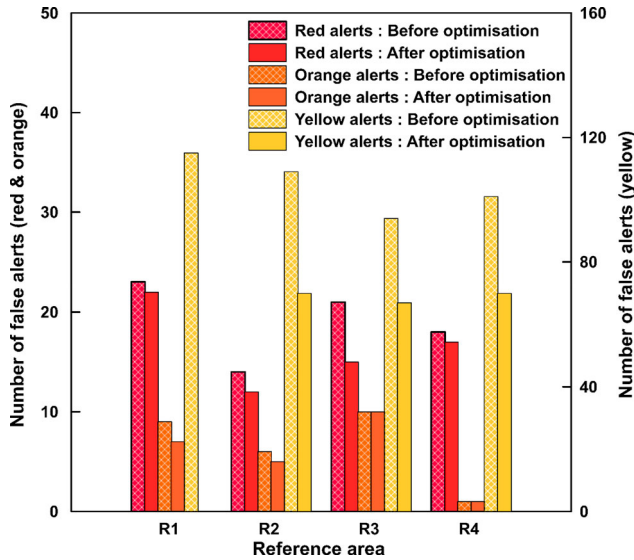
Figure 8. Number of false alarms before and after optimization.
