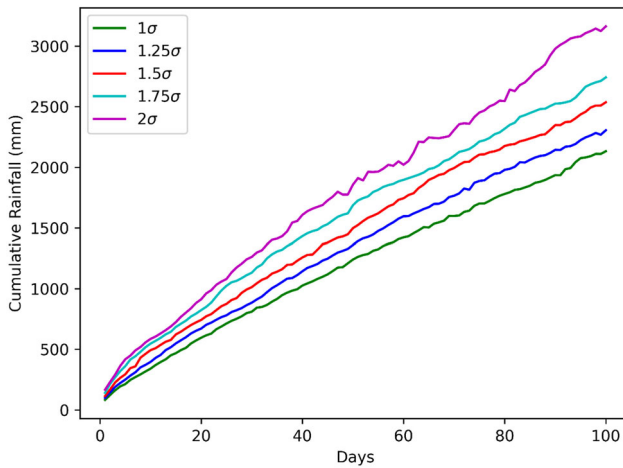
Figure 5. An example of threshold curves for cumulative rainfall up to 100 days; ‘ \sigma ’ is the standard deviation of each series.
