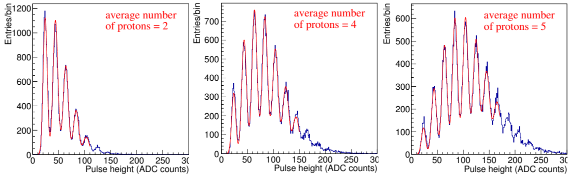
Figure 8. Acquired spectra for different average multiplicities (2, 4 and 5, respectively) of proton per pulse.
