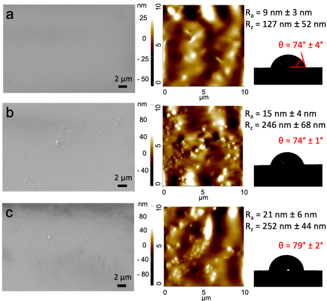
Figure 4. SEM and AFM images of pristine paint (a); HNT-SA/paint and (b); HNT-TCPM/paint coatings (c) with the corresponding optical micrographs of water contact angle. The reported roughness values are the average of 3 maps acquired on different regions of the
