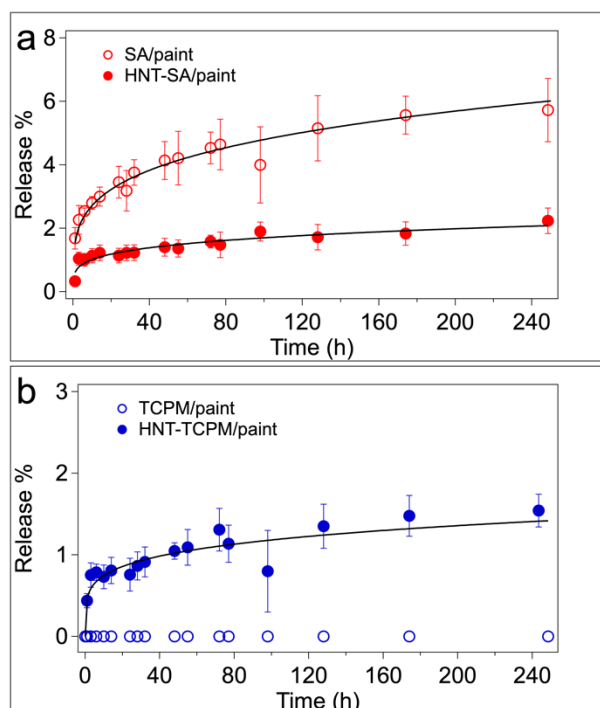
Figure 5. Release kinetic profiles of SA- (a) and TCPM (b) from the composites. Markers represent the average calculated on 3 experimental measurements \pm standard deviation; the corresponding fitting curves were calculated according to Korsmeyer-Peppas equation.
