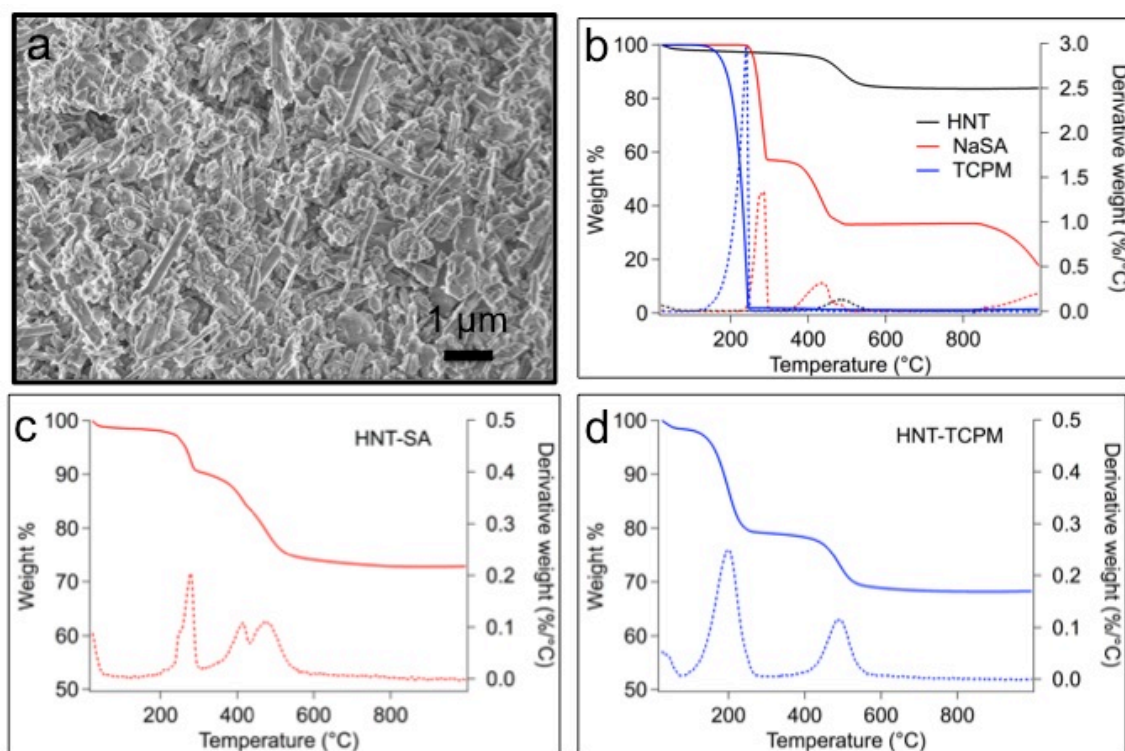
Figure 2. SEM image of pristine HNTs Imerys (a); TG curves of pristine HNTs, SA and TCPM (b), HNTs loaded with SA in water at pH \approx 8 (c), and HNTs loaded with TCPM in DMSO (d).
