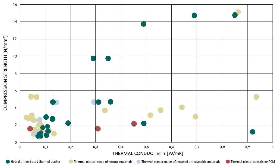
Figure 1. Thermal plasters investigated and compared considering the relation between the compression strength \sigma (N/mm 2 ) and the thermal
