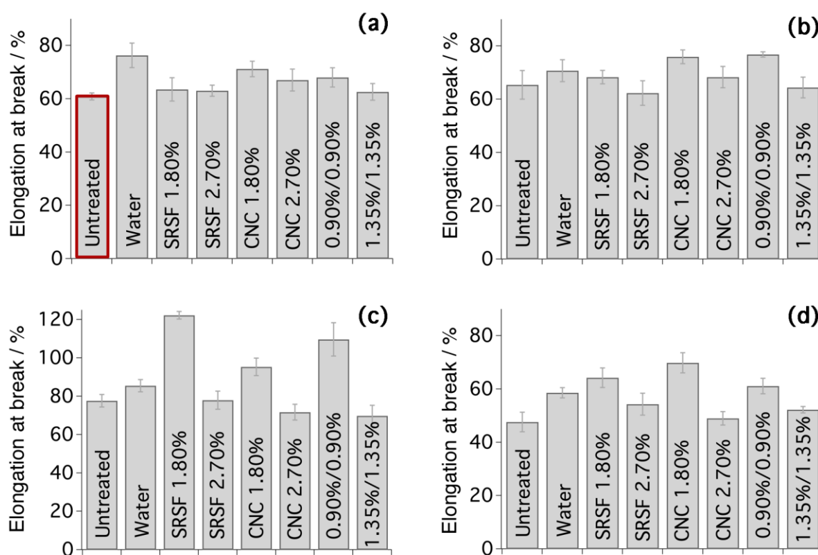
Figure S3. Elongation at break of pristine (a) and aged silk mockups, namely AS1 (b), AS2 (c) and AS3 (d), treated with water, SRSF, CNC and hybrid systems at different concentrations. Untreated silk, used as a reference, is included in each graph. The hybrid formulations maintained the original elongation of pristine silk fibers (red boxed bar in panel a).
