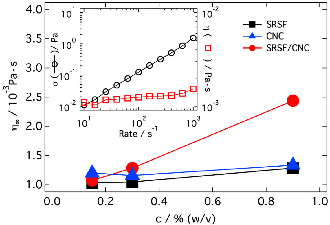
Figure 3. High-shear viscosity \eta_\infty measured at 0h for SRSF (full squares), CNC (full triangles) and SRSF/CNC (full circles) dispersions with concentration 0.15%, 0.30% and 0.90% w/v. Inset: Stress \sigma (open circles) and viscosity \eta (open squares) vs. rate for an example of flow curve (SRSF 0.90%). The value of \eta_\infty was extracted from the data region corresponding to rate values comprised between 10^2 and 5 \times 10^2 \text{ s}^{-1} . Error bars are smaller than markers.
