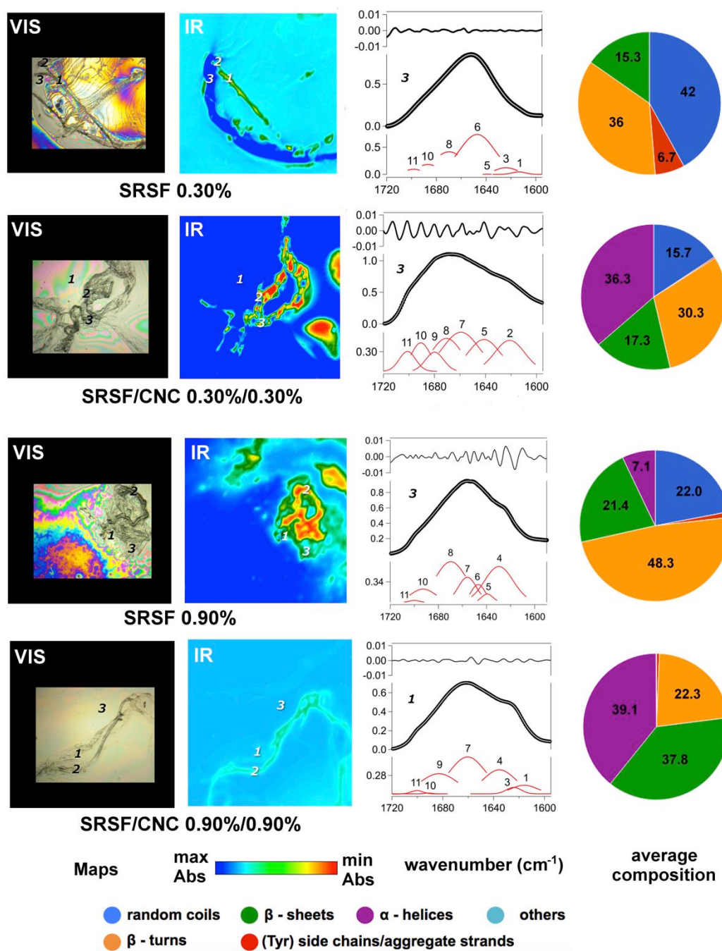
Figure 4. Films cast from SRSF (0.30%, 0.90% w/v) and SRSF/CNC (0.30%/0.30%, 0.90%/0.90% w/v) dispersions on Au sputtered glass slides. The visible (VIS) and infrared (IR) maps show areas of 700 x 700 \mu\text{m}^2 ; in the false color IR maps, the intensity of the films' spectra at 1620 \text{cm}^{-1} (aggregate \beta -strand/intermolecular \beta -sheets, weak) is imaged, using the chromatic scale: red > yellow > green > blue. Numbers on the maps indicate locations where the acquired spectra were deconvoluted to investigate the secondary structure of fibroin. For each film, a representative spectrum of one such location is shown in the 1720-1690 \text{cm}^{-1} region, along with the Amide I
