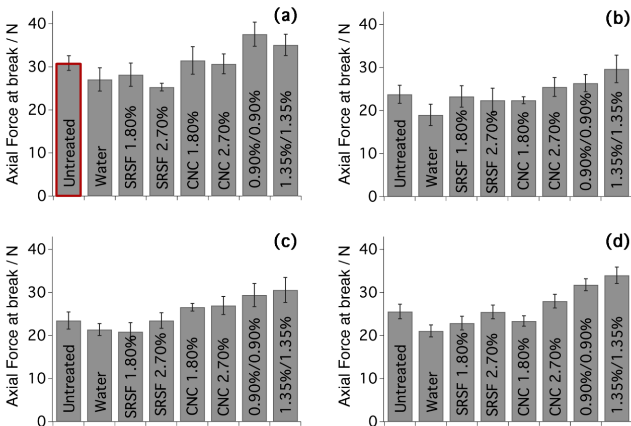
Figure 5. Axial force at break of pristine (a) and aged silk mockups, namely AS1 (b), AS2 (c) and AS3 (d), treated with water, and with SRSF, CNC and hybrid SRSF/CNC formulations at different concentrations. Untreated silk (i.e. pristine or aged samples where formulations were not applied) is included as a reference in each graph. The hybrid formulations restored the axial force at break of the aged silk back to that of pristine silk (red boxed bar in panel a).
