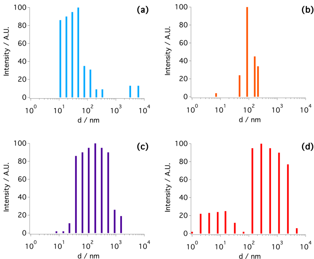
Figure 1. DLS intensity-weighted plots measured for (a) SRSF (1.80% w/v), (b) SRSF/CNC (0.30%/0.30% w/v), (c) SRSF/CNC (0.90%/0.90% w/v) and (d) CNC (1.80% w/v) right after the preparation.
