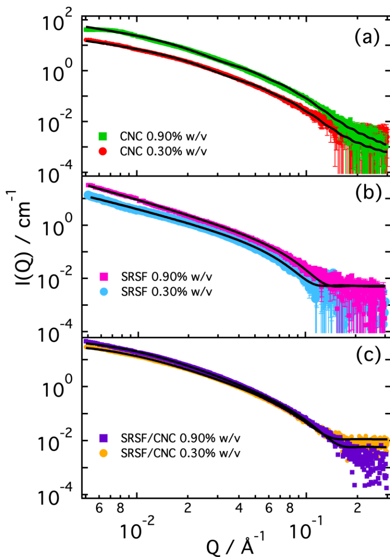
Figure 2. SAXS spectra measured for (a) CNC (0.90%, 0.30% w/v, as indicated), (b) SRSF (0.90%, 0.30% w/v, as indicated), and (c) SRSF/CNC (0.90%/0.90%, 0.30%/0.30% w/v, as indicated) dispersions right after their preparation. Lines in (a) are fits of a parallelepiped form factor model, while lines in (b) and (c) are fits of a mass fractal model. The fitting parameters are reported in Table S1 and Table 1, respectively.
