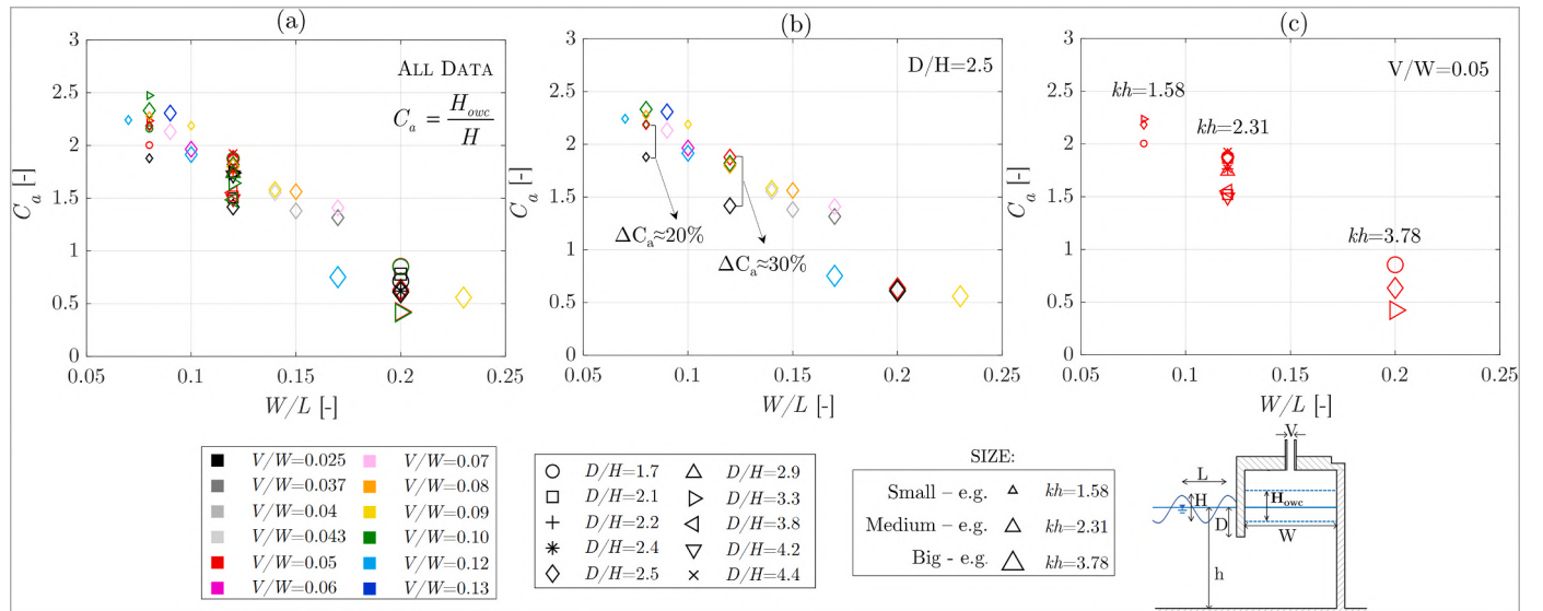
Fig. 14. Variation of the OWC absorption coefficient C_a versus W/L for the whole dataset (a), cases with D/H = 2.5 only (b) and cases V/W = 0.05 only (c).
