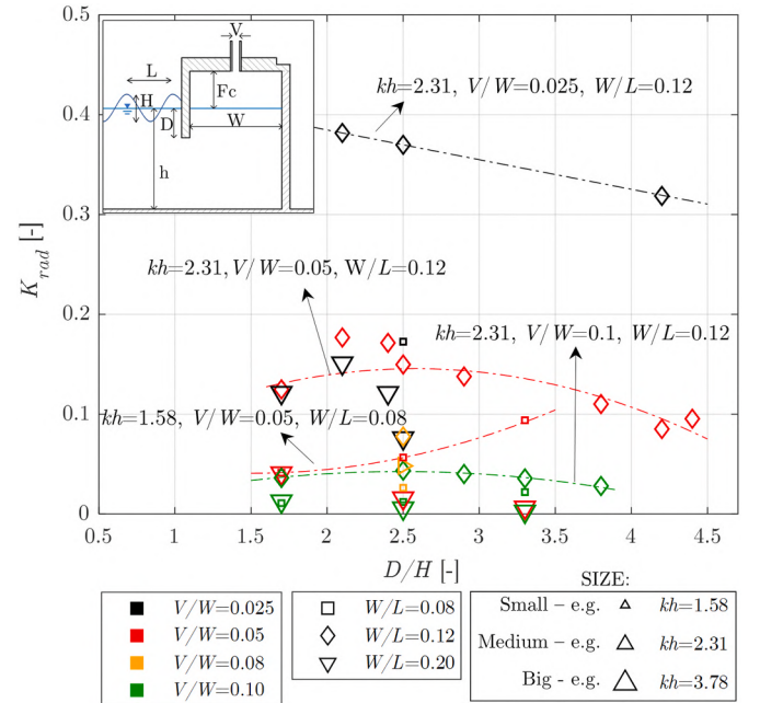
Fig. 12. Variation of radiation coefficient ( K_{rad} ) versus D/H . For the sake of readability, results are shown only for W/L = 0.08 , W/L = 0.12 and W/L = 0.20 .
