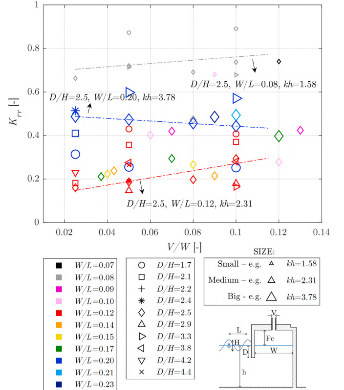
Fig. 7. Variation of total reflection coefficient ( K_{rr} ) versus relative top-cover aperture V/W .
