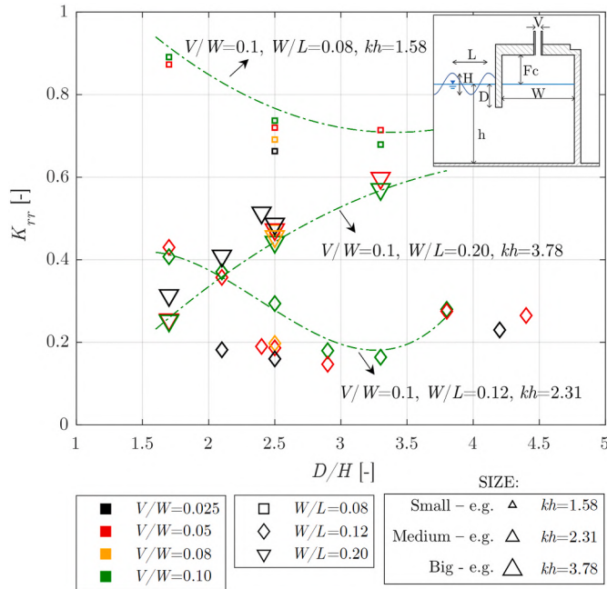
Fig. 6. Variation of total reflection coefficient ( K_{rr} ) versus relative front wall draught D/H . For the sake of readability, results are shown only for W/L = 0.08 , W/L = 0.12 and W/L = 0.20 .
