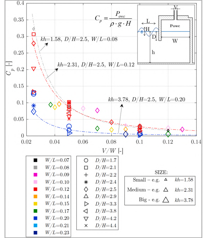
Fig. 15. Variation pressure coefficient C_p versus V/W .
