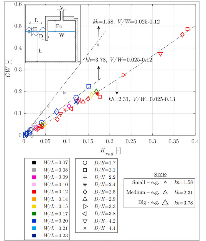
Fig. 17. Variation of the OWC capture width ratio CW versus K_{rad} .
