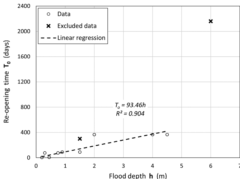
FIGURE 3 Depth-idleness vulnerability function for cultural heritage. Two points have been excluded from the regression
