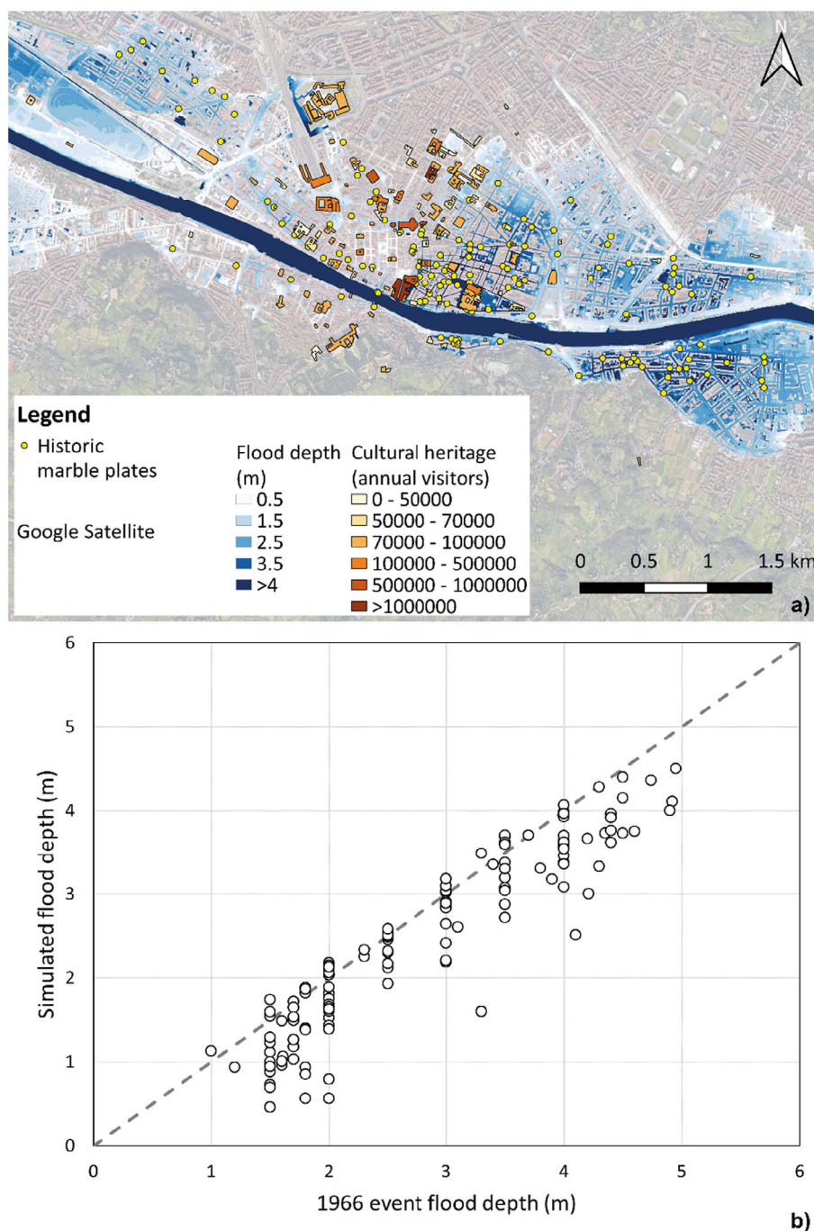
FIGURE 4 Flood hazard results. (a) 500 years flood depths, CH exposure and location of historical marble plates, (b) validation of flood hazard model against the historical flood depths
