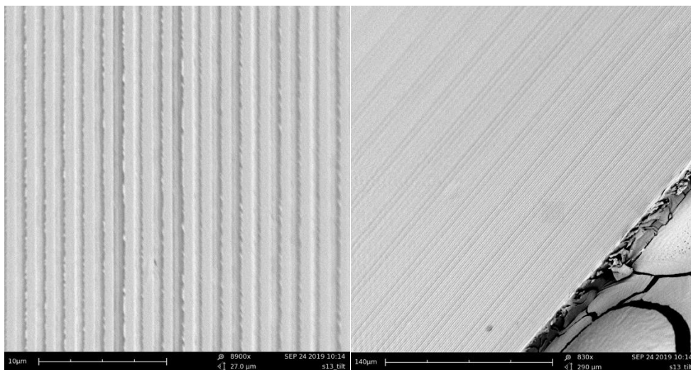
Figure 3.6: Scanning electron microscope photograph of the PEGDA-based patterns obtained through soft lithography from PDMS mold. The scale bar in the left-hand-side image is 10 \mu\text{m} , while in the right-hand-side one is 140 \mu\text{m} .
