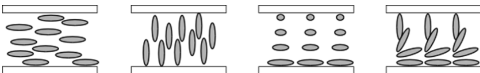
Figure 1.5: Different alignments of LC molecules in a cell. From left to right: planar homogeneous, homeotropic, twisted and splayed alignment.
