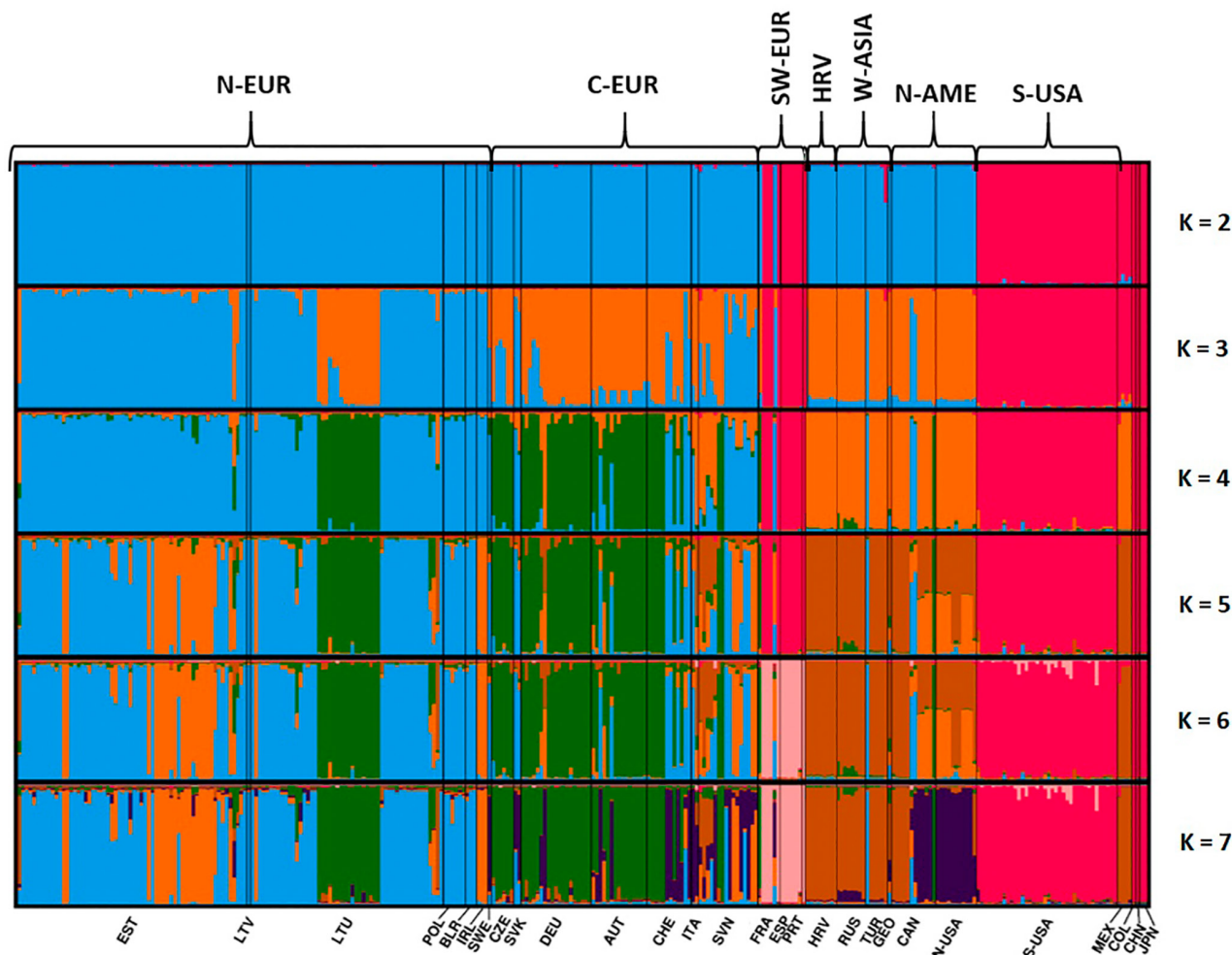
FIGURE 4 STRUCTURE clustering of the Lecanosticta acicola clone-corrected dataset, representing K = 2 – 7 . Optimal number of clusters ( K = 2 ) by \Delta K and ( K = 7 ) by \ln(\text{Pr}(X|K)) . Population codes are displayed under the figure; above the figure division into regions as analysed in the migration analyses is displayed. Definition of population codes: AUT, Austria; BLR, Belarus; CAN, Canada; CHE, Switzerland; CHN, China; COL, Colombia; CZE, Czech Republic; DEU, Germany; ESP, Spain; EST, Estonia; FRA, France; GEO, Georgia; HRV, Croatia; IRL, Ireland; ITA, Italy; JPN, Japan; LTU, Lithuania; LTV, Latvia; N-USA, north-eastern United States; MEX, Mexico; POL, Poland; PRT, Portugal; RUS, Russia; S-USA, south-eastern United States; SVK, Slovakia; SVN, Slovenia; SWE, Sweden; TUR, Turkey.
