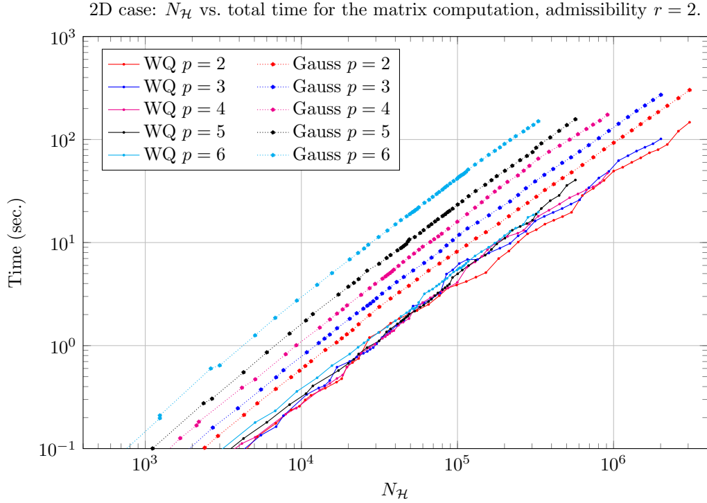
Figure 4: L^2 -projection: N_{\mathcal{H}} vs. total time for the matrix computation for the 2D case and admissibility parameter r = 2 . For WQ the total time for the matrix computation is the sum of the time needed for the preprocessing (Section 3.2) and for the matrix formation (Section 3.3).
