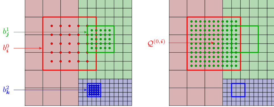
Figure 2: Example of a hierarchical mesh with three different levels. Three basis functions from \mathcal{B}^\ell , with \ell = 0, 1, 2 are considered. The supports and quadrature points for these B-splines from spaces \mathcal{B}^0 (red), \mathcal{B}^1 (green) and \mathcal{B}^2 (blue) are depicted on the hierarchical mesh (left). The quadrature points for b_i^0 \in \mathcal{H} used in weighted quadrature for hierarchical B-splines are also shown (right).
