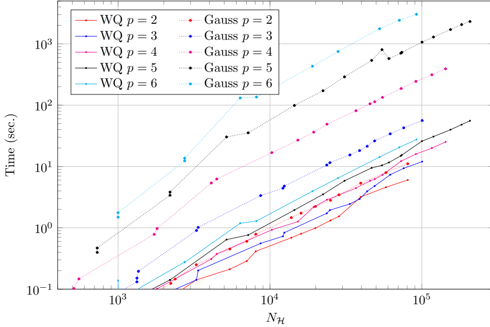
Figure 9: L^2 -projection: N_{\mathcal{H}} vs. total time for the matrix computation for the 3D case and admissibility parameter r = 2 . For WQ the total time for the matrix computation is the sum of the time needed for the preprocessing (Section 3.2) and for the matrix formation (Section 3.3).
