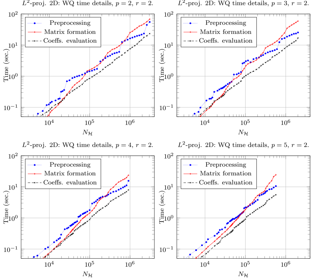
Figure 6: N_{\mathcal{H}} vs. the CPU time needed to run the WQ algorithm: preprocessing (Algorithm 3) and matrix computation (Algorithm 5) for the L^2 -projection in 2D and admissibility parameter r = 2 . The cost for the matrix computation is split in the CPU cost for coefficient evaluations ((32) for n = 0, \dots, L ) and the CPU cost for executing the rest of the Algorithm 5.
