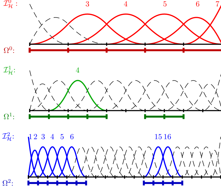
Figure 1: An example of an univariate hierarchical space. Mesh cells and B-splines for levels 0,1,2 are depicted in top, middle and bottom plot, respectively. The hierarchical space is determined by domains \Omega^\ell , its basis functions in \mathcal{I}_\mathcal{H}^\ell are marked and labeled in each plot.
