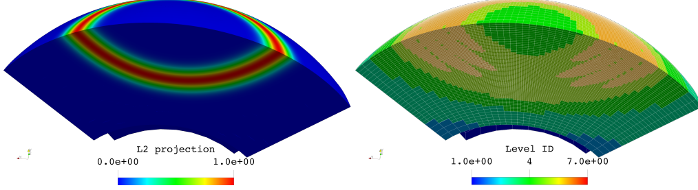
Figure 8: L^2 -projection (left) and element levels (right) after 27 adaptive refinements for the 3D case with degree p = 2 and admissibility r = 2 . For this configuration the space contains 754614 degrees of freedom, and the L^2 -error between the function (45) and its L^2 -projection is \approx 8.5e - 6 .
