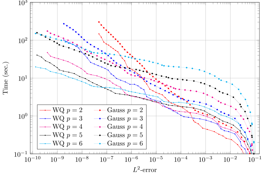
Figure 5: L^2 -projection: L^2 -error vs. total time for the matrix computation for the 2D case and admissibility parameter r = 2 . For WQ the total time for the matrix computation is the sum of the time needed for the preprocessing (Section 3.2) and for the matrix formation (Section 3.3).
