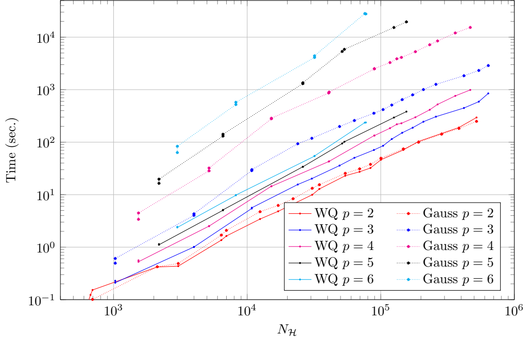
Figure 12: Linear elasticity: N_{\mathcal{H}} vs. total time for the matrix computation in the 3D case and admissibility parameter r = 2 . For WQ the total time for the matrix computation is the sum of the time needed for the preprocessing (Section 3.2) and for the matrix formation (Section 3.3).
