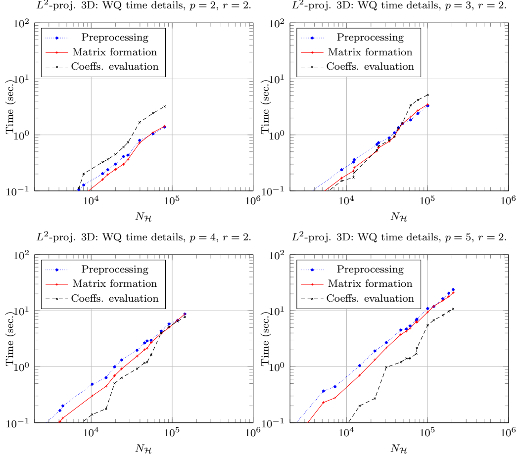
Figure 11: N_{\mathcal{H}} vs. the CPU time needed to run the WQ algorithm: preprocessing (Algorithm 3) and matrix computation (Algorithm 5) for the L^2 -projection in 3D and admissibility parameter r = 2 . The cost for the matrix computation is split in the CPU cost for coefficient evaluations ((32), for n = 0, \dots, L ) and the CPU cost for executing the rest of the Algorithm 5.
