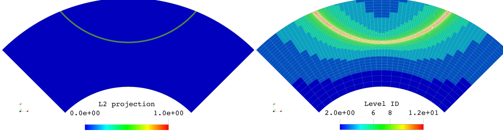
Figure 3: L^2 -projection (left) and element levels (right) after 51 adaptive refinements for the 2D case with degree p = 2 and admissibility r = 2 . For this configuration the space contains 867947 degrees of freedom, and the L^2 -error between the function (45) and its L^2 -projection is \approx 3.4e - 7 .
