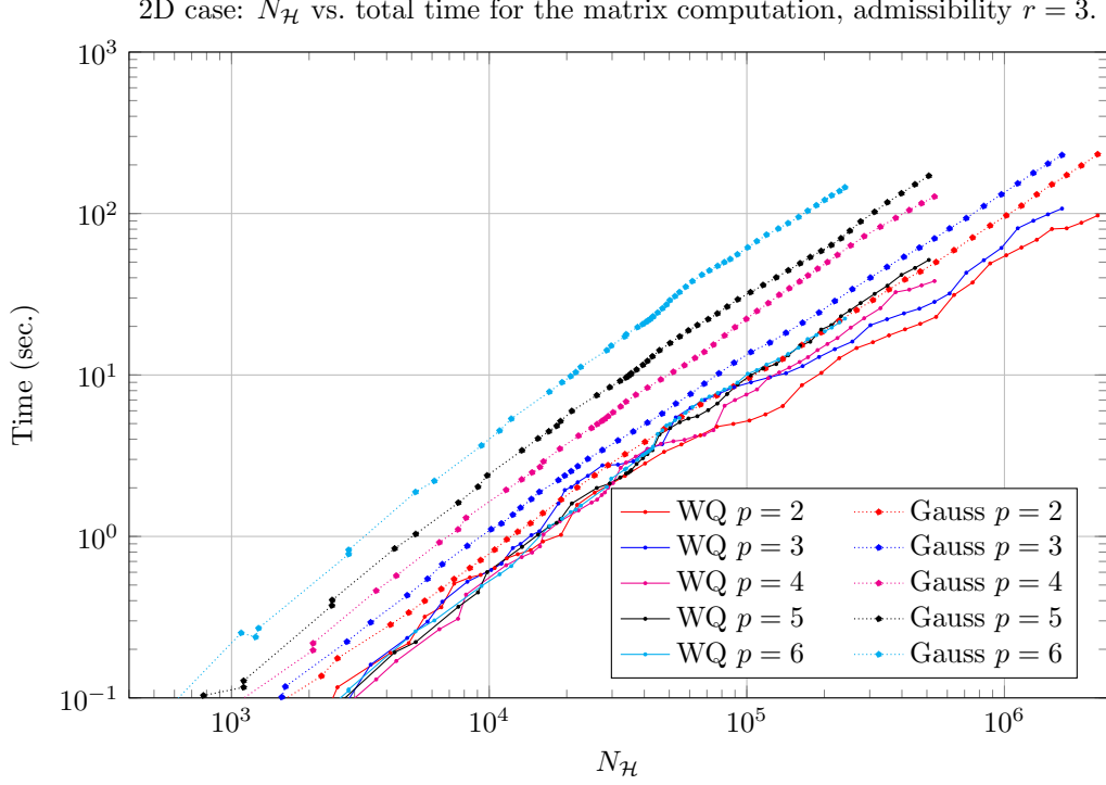
Figure 7: N_{\mathcal{H}} vs. total time for the matrix computation for the 2D case and admissibility parameter r = 3 . For WQ the total time for the matrix computation is the sum of the time needed for the preprocessing (Section 3.2) and for the matrix formation (Section 3.3).
