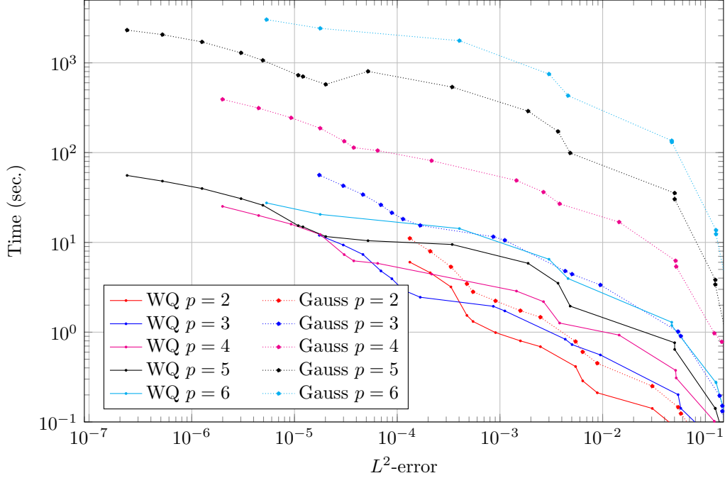
Figure 10: L^2 -projection: L^2 -error vs. total time for the matrix computation for the 3D case and admissibility parameter r = 2 . For WQ the total time for the matrix computation is the sum of the time needed for the preprocessing (Section 3.2) and for the matrix formation (Section 3.3).
