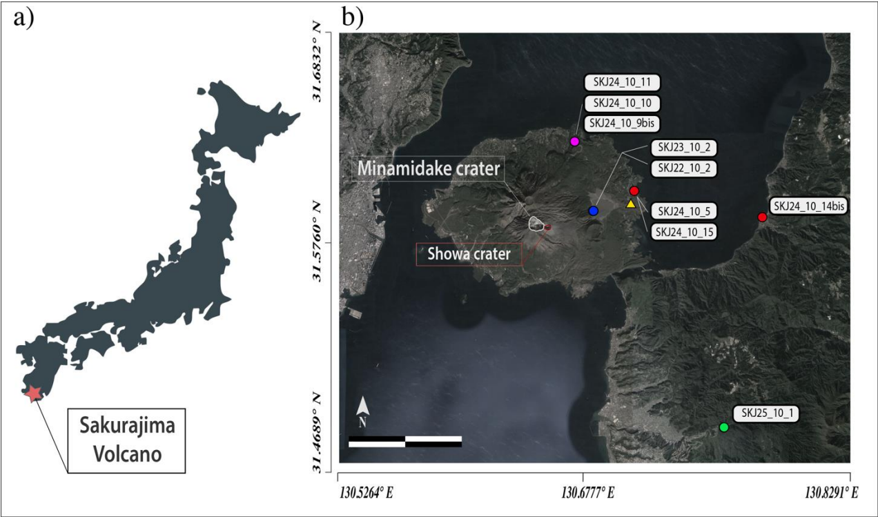
Fig. 1 (a) Location of Sakurajima volcano indicated within a sketch map of the Japan archipelago; (b) locations of the ash samples (indicated with circles) reported in the map with variable colors according to the different stages observed in the eruptive activity: Weak Ash Emission (blue circle), Vulcanian Explosion (red circles), Continuous ash venting (violet circle), and activity renewal (green circle). The yellow triangle marks the site of the thermal camera video recording (31.588974° N 130.707363 °E).
