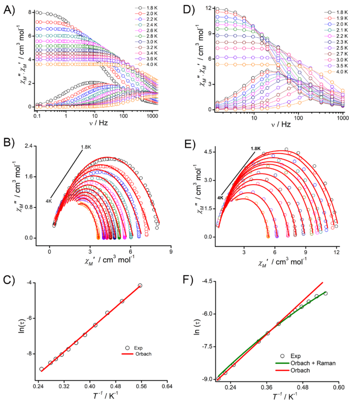
Figure 5. Frequency-dependent ac susceptibility measurements were performed on polycrystalline samples of 5\text{-Tb} and 6\text{-Dy} at the indicated temperatures ( H_{ac} = 3.5 Oe) in the absence of an external field. Panels (A–C) represent in-phase/out-of-phase vs frequency, Cole–Cole, and the Arrhenius plots, respectively, for the complex 5\text{-Tb} , while panels (D–F) correspond to 6\text{-Dy} . The solid red curves in panels B and E represent the best fit obtained using the generalized Debye model. The solid red line in panel C and F represent the linear fit, and the solid green line in panel F represent the nonlinear fit (Orbach + Raman) of the experimental data.
