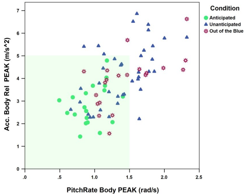
Figure 5. Scatter plot of the peaks of the kinematic parameters of the upper-body response for automatic braking of 5L profile for the three aware conditions tested. (Magnitudes from the tests, without controlling AB-decel and AB-jerk ). The shaded area covers all responses with anticipated AB.
