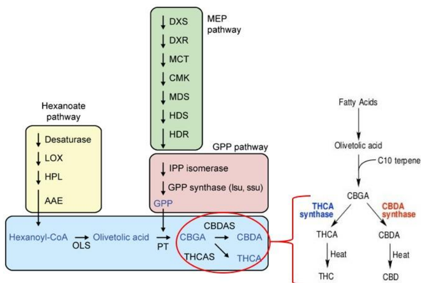
Figure 3. The phytocannabinoids biosynthesis pathway in cannabis and its related gene networks [12]. Heating will immediately decarboxylate THCA and CBDA into THC and CBD making them readily available for use by your body.
