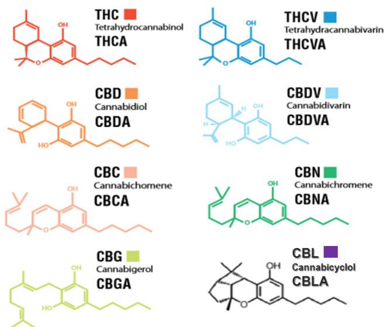
Figure 1. Natural important cannabinoids and their structure.
