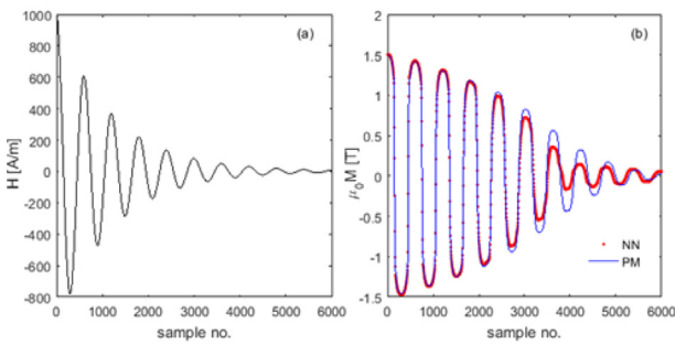
Fig. 14. Simulations of the DATASET 5: magnetic field sequence (a) and magnetic polarization sequences (b) calculated by both the PM and the NN-based model.
