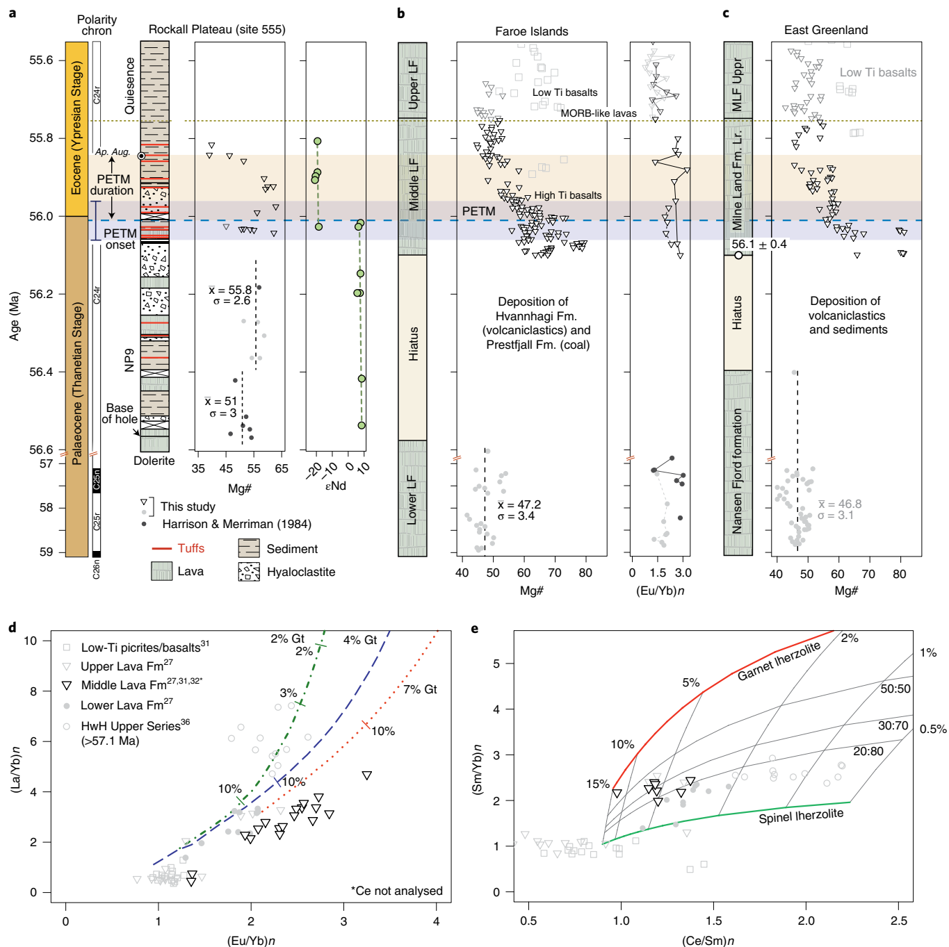
Fig. 2 | Palaeocene-Eocene volcanostratigraphy and geochemistry of the proto-northeast Atlantic ridge. a , Simplified log of the Rockall ‘Phase 1’ sequence 19 showing lithologies, Mg# (that is, 100 \times \text{molecular MgO}/(\text{MgO} + \text{FeO}) , where FeO is assumed to be 0.9\text{FeOT} ) and \epsilon Nd (Extended Data Fig. 1). Please note the scale break at 56.6 Ma; the vertical dashed lines in panels (a) to (c) show mean ( \bar{x} ) values for variables over the intervals shown. b,c , Simplified log of the Faroes Basalt formations 26 (b), with Mg# and (Eu/Yb)_n (chondrite-normalized 56 ); Mg# data are from ref. 26 and (Eu/Yb)_n are from refs. 27,32 (Extended Data Fig. 2); note the sharp transition to high Mg# (and enriched rare earth element contents) at ca. 56.1 Ma, which is also observed in east Greenland (Milne Land Formation) 26 MORB, mid-ocean ridge basalt; Fm., formation. (c). d , (La/Yb)_n versus (Eu/Yb)_n of the Faroes and Hold with Hope (HwH) lavas (chondrite-normalized 56 ) and modelled non-modal batch melting of a lherzolitic mantle source, adopted from ref. 33 , showing different degrees of melting of a garnet lherzolite (green, blue and red curves). e , (Sm/Yb)_n versus (Ce/Sm)_n and a rare earth element melting model (Methods), showing percentage melt along the top and the relative proportions of garnet- and spinel-lherzolites from 100% gt-lherzolite (red curve) to 100% sp-lherzolite (green curve). Both models indicate that the Faroes Middle Lava Formation (that is, high-Mg# basalts in the lower 500 m of the Middle Lavas; see b), which erupted immediately before and during the PETM, experienced the highest degrees of melting of a mantle source containing \geq 10\% garnet.
