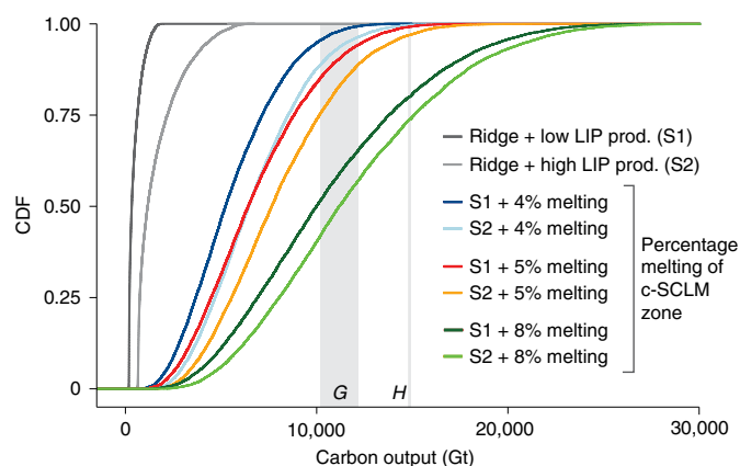
Fig. 3 | Simulations of volcanic carbon release during the PETM. Results are plotted as cumulative distribution functions (CDFs). The grey lines show the estimated carbon output from ridge volcanism and LIPs alone; with S1 and S2 showing low (0.6 km 3 per year) and high (2.4 km 3 per year) LIP volcanic productivity (prod.) scenarios 4 , respectively (Extended Data Fig. 4 and Methods). The coloured lines show the effects of adding 4% to 8% carbonated (c-) SCLM melt along the incipient ridge during breakup. The grey vertical bars denote the carbon output necessary to drive and sustain PETM warming estimated by Gutjahr et al. 11 (labelled G; 10,200–12,200 Gt C) and Haynes and Hönisch 13 (labelled H; 14,900 Gt C).
