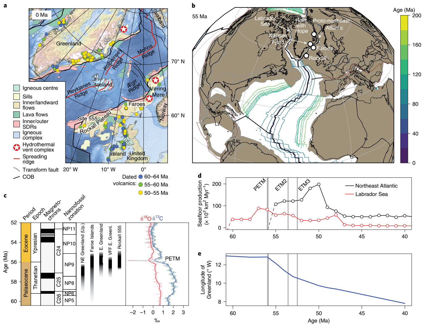
Fig. 1 | Early Cenozoic tectonic and magmatic evolution of the northeast Atlantic. a , Map of the present day northeast Atlantic region showing the distribution of Palaeocene–Eocene lava flows and intrusives, with dated volcanics denoted by coloured symbols and the locations of major hydrothermal vent complexes in the Vøring and Møre Basins 15 and offshore Northeast Greenland 54 shown as stars (SDRs = seaward-dipping reflectors; COB = continent–ocean boundary). b , Plate tectonic reconstruction showing nascent ridge systems developing along the Labrador Sea and northeast Atlantic at 55 Ma; the perimeter to brown shaded regions shows continent–ocean boundaries, and brown lines signify subduction zones (Methods). c , Ages of the volcanic sections discussed (Up. = Upper; VFF = Vandfaldsdalen Fm, E. = East, Green. = Greenland), defined by radiometric dates 12 , magnetostratigraphy and nanofossil zonation 22,25,37 and corresponding carbon and oxygen isotope records showing the PETM isotope excursions (solid and faint lines show 1 Myr and 20 kyr locally weighted functions, respectively). d , Seafloor production rates for the Labrador Sea and northeast Atlantic, derived from GPlates (Methods), shown alongside the timing of Eocene hyperthermals (PETM and Eocene Thermal Maximum (ETM) 2 and 3). e , Palaeolongitude of Greenland 7 , indicating the onset of ocean crustal production in the Northeast Atlantic at 56 Ma. Panel a is adapted with permission from ref. 3, Springer Nature Limited.
