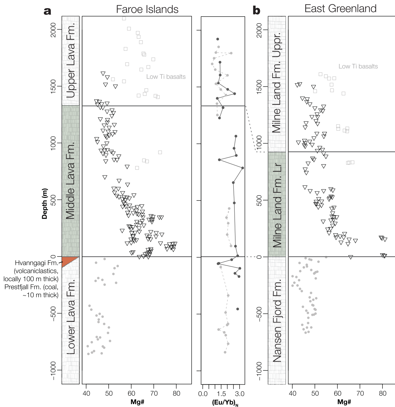
Extended Data Fig. 2 | Compositional characteristics of lavas from the Faroes and Greenland. Simplified log of basalt lava successions from the Faroes and east Greenland (modified after ref. 26 , with Mg# and (Eu/Yb)_N (chondrite-normalised 26 ); Mg# data are from ref. 26 and (Eu/Yb)_N are from refs. 27,32 .
