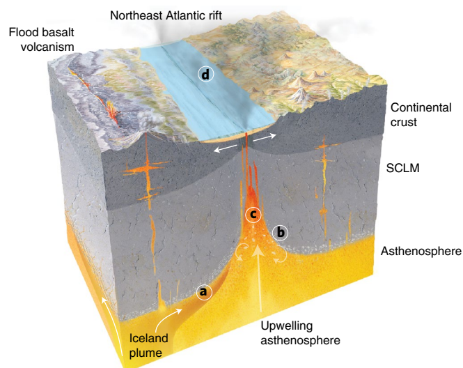
Fig. 4 | Deep carbon mobilization and release in the North Atlantic during the PETM. The model stages are shown. a , Thermomechanical weakening of the SCLM by the Iceland plume. b , Thermal removal, delamination and lateral advection of metasomatized SCLM (shown as the white stippled pattern) by edge-driven convection in the asthenospheric mantle. c , Carbonate-rich domains are entrained into the central melt zone beneath the evolving rift, where they are thermodynamically unstable and involved in transient decompression melting just before continental breakup. d , Massive outgassing of CO 2 at Earth's surface from the northeast Atlantic rift and associated volcanic and tectono-magmatic systems. Credit: Gary Hincks.
