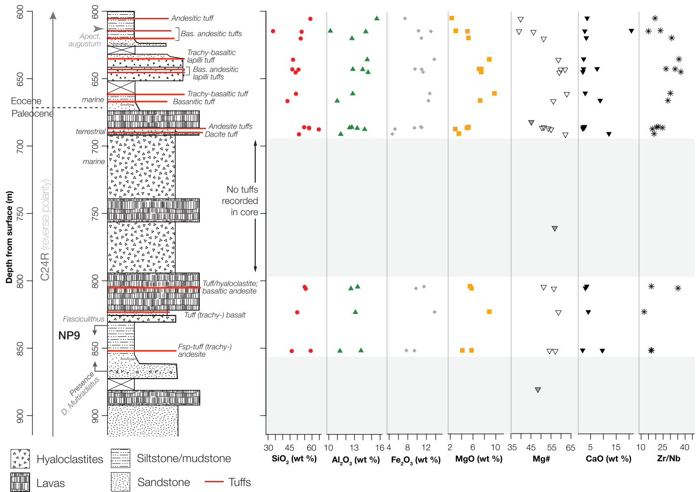
Extended Data Fig. 1 | Schematic stratigraphic log of Palaeocene-Eocene volcanic and sedimentary lithofacies at DSDP Leg 81 Site 555, and the composition of tuff layers. The corresponding plots show the major-element composition, and Mg#, of tuff layers, shown as horizontal red lines (and labelled by lithology; see also Extended Data Fig. 3a) on the log. The Mg# of a number of basalt lavas and tuffs from Harrison and Merriman 99 are also shown as filled grey symbols.
