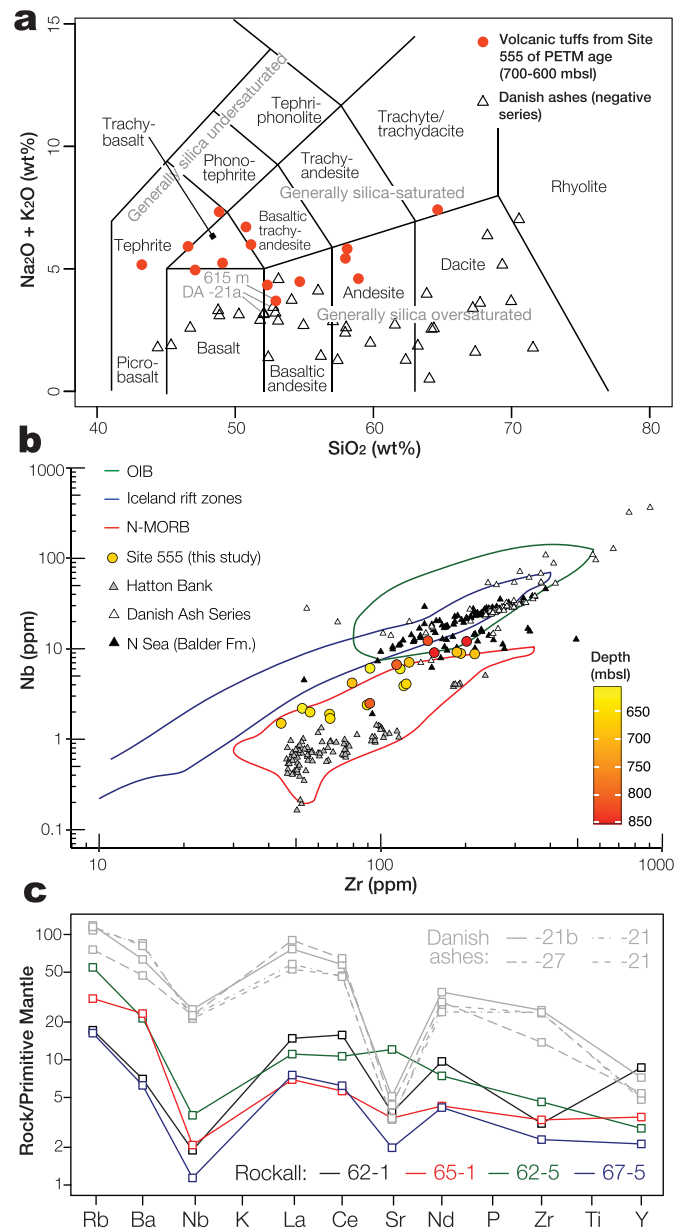
Extended Data Fig. 3 | Geochemical characteristics of tuffs layers from DSDP Leg 81 Site 555. Total alkali-silica (TAS) diagram (after ref. 101 ) showing the composition of volcanic tuffs of PETM age (approximately 700-600 mbsl; see Extended Data Fig. 2), in addition to Danish ashes of the 'negative series' 23 . b, Nb versus Zr of tuffs from Site 555, shown alongside tuffs of the Danish Ash Series 23 and Balder Formation in the North Sea 102 , and lavas from the Rockall/Hatton Bank 103 . The fields shown for OIB, N-MORB and Iceland rift-zones are from ref. 104 . c, Incompatible element patterns of Rockall tuffs from the upper section (700-600 mbsl) normalized to primitive mantle 105 . The corresponding depths in the core are provided in Extended Data Table 3. For comparison, some Danish ashes (negative series) are also shown 23 .
