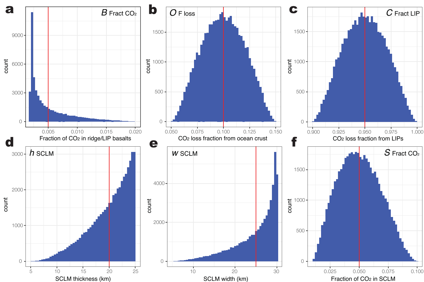
Extended Data Fig. 4 | Input distributions for sampled variables used in carbon outgassing simulations. a, Fraction of CO 2 present in mid-ocean ridge basalts and those of large igneous provinces (LIPs); b, Fraction of CO 2 lost from the ocean crust via degassing at mid-ocean ridges; c, Fraction of CO 2 lost from LIP basalt eruptions; d, Thickness of the sub-continental lithospheric mantle (SCLM); e, Width of the SCLM melting zone beneath the mid-ocean ridge system; f, Fraction of CO 2 present in the SCLM. Note that the red line denotes the mean. See the Methods for further information on these variables.
