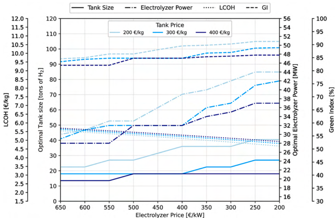
Fig. 18. Tank and electrolyzer price effect on the variation on optimal configuration parameters: LCOH (dotted line), GI (dashed line), tank size (continuous line) and electrolyzer size (dash-dotted line).
