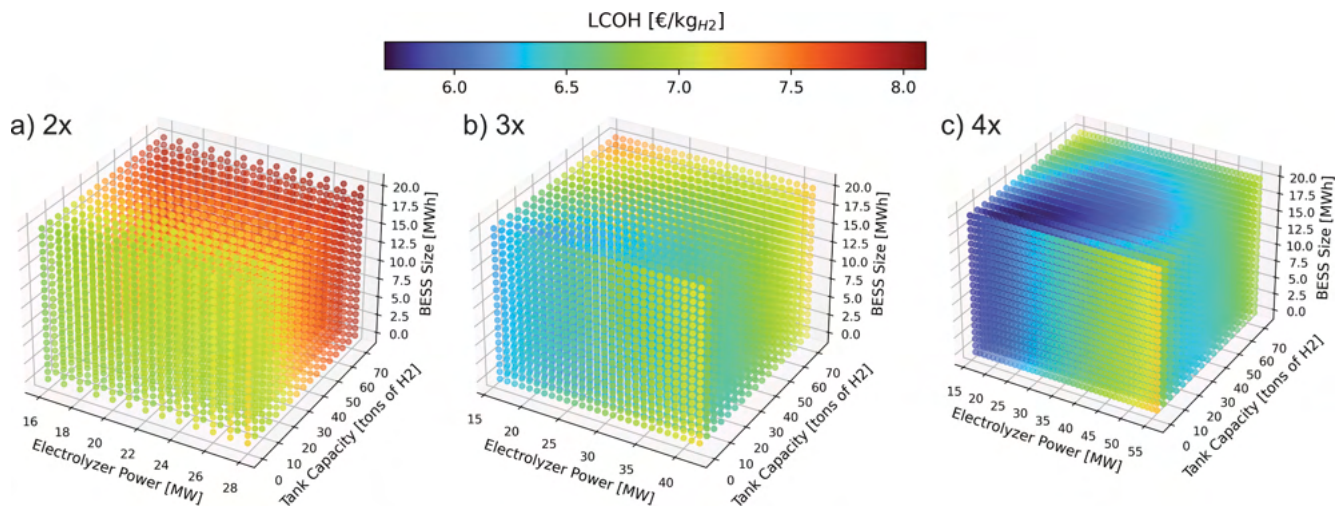
Fig. 12. LCOH indicators varying BESS capacity, tank capacity and electrolyzer power. Comparison among different wind farm size scales. All graphs use the same color scale.
