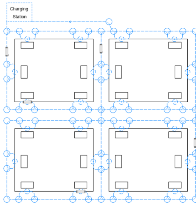
Figure 3: Plant layout.
