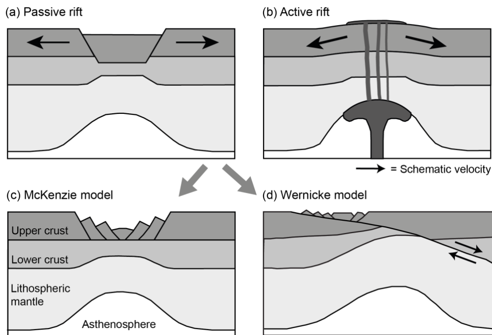
Figure 4: Conceptual rift models. (a) Far-field forces related to plate tectonics (such as the pull of subducting slabs) cause continental extension in the passive rifting model. The name of the concept emphasises the passive role played by the mantle. (b) In active rifting, an active upwelling of warm mantle material causes volcanism and surface uplift. The plates glide gravitationally away from the uplift, thus leading to extension. (c) The McKenzie model (a form of passive rifting) envisages thinning of the upper crust, lower crust and lithospheric mantle in a pure shear mode (McKenzie, 1978). (d) In the Wernicke model (also a form of passive rifting), simple shear deformation along a low-angle detachment fault causes thinning of the upper crust that is offset from thinning of the lower crust (Wernicke, 1985).
