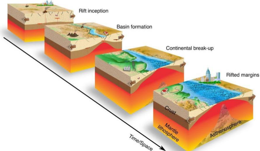
(c) Conceptual evolution of continental rifting
