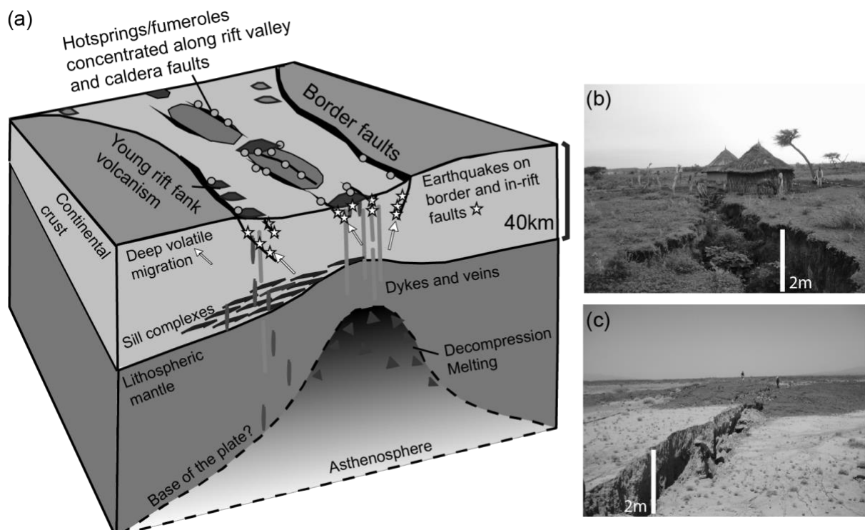
Figure 7: Earthquakes and geothermal potential of rifts. (a) Cartoon sketch of a magnetically active continental rift showing zones of surface faulting and volcanism, and the subsurface processes associated with these. (b) Photos of discrete and sudden fissuring and faulting events associated with rainfall induced subsidence and (c) earthquake swarms. Photos by Derek Keir.
