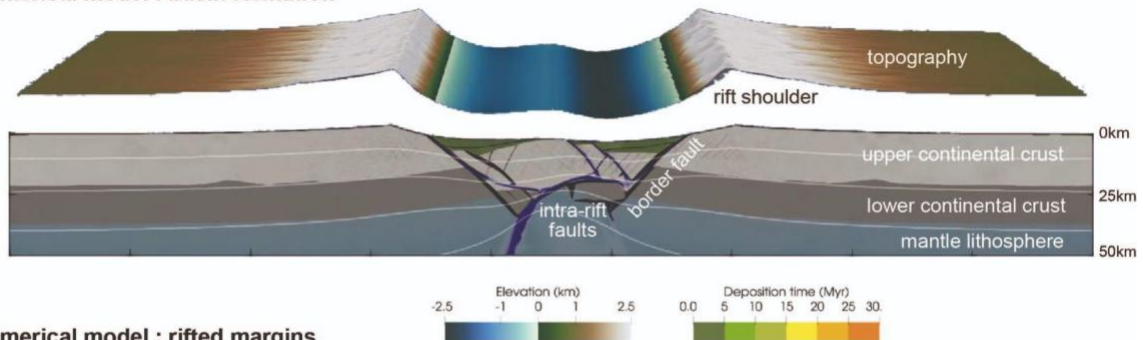
(b) Numerical model : rifted margins
