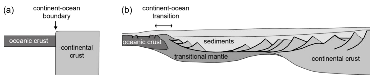
Figure 5: Concepts of rifted margin architecture. (a) Early studies depicted the transition from continent to ocean as abrupt. This view juxtaposes continental to oceanic crust along what can be mapped as a continent-ocean boundary line. Inspired by Wegener (1912). (b) Modern views see the transition from continent to ocean as gradual, encompassing tilted continental blocks and regions of exhumed and altered mantle. This view implies a continent-ocean transition zone, rather than a boundary. Redrawn from Peron-Pinvidic et al. (2013) with permission from Elsevier.
