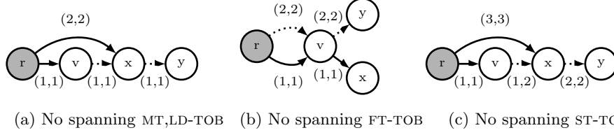
Fig. 3: Examples of temporal graphs that do not admit a spanning D-TOB with root r . Solid arcs represent a maximum D-TOB.
