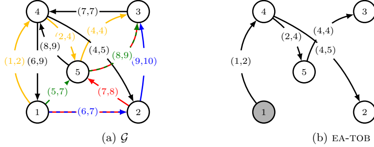
Fig. 1: (a) Temporal graph with different walks from vertex 1 to vertex 3, each one represented by a color (two-tone arcs belong to two walks). Yellow : walk realizing EA(1, 3) . Green : walk realizing MT(1, 3) . Blue : walk realizing both ST(1, 3) and LD(1, 3) . Red : walk realizing FT(1, 3) . (b) An EA-TOB of \mathcal{G} with root 1.
