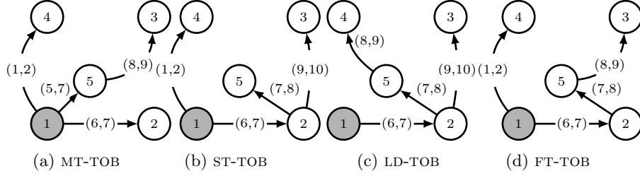
Fig. 2: Example of D-TOBs of the temporal graph \mathcal{G} in Figure (1a) for different distances. The grey vertex is the root of the TOB.
