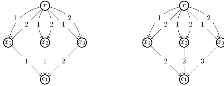
(a) All temporal arcs have elapsed time 0. (b) All temporal arcs have elapsed time 1.
