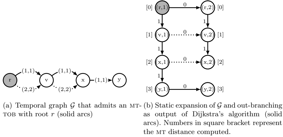
Fig. 4: Example when the Dijkstra's algorithm on the static expansion present parities between vertices but only one choice leads to a TOB.
