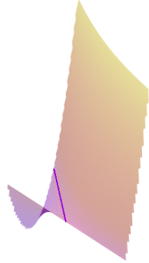
FIGURE 5. The surface \Sigma_{\pi/3, \pi/6}^+ with \beta = \alpha + \pi . The existence of K is granted by Corollary 4.7.
