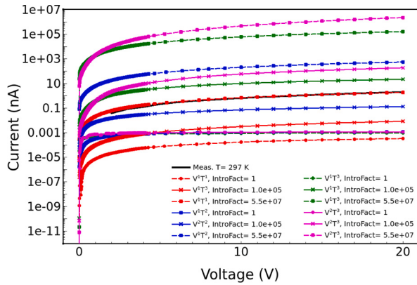
Fig. 8. Simulated I-V curves vs. measurements ( 20\text{ }^{\circ}\text{C} ): effects of temperature, voltage and introduction factor.
