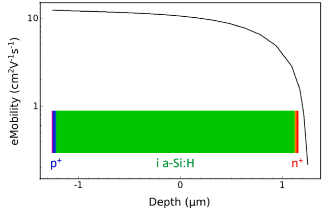
Fig. 6. Carriers mobility map within a reference p-i-n device on kapton.
