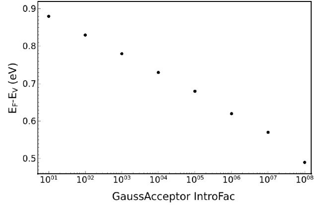
Fig. 5. Fermi's level position variation as a function of the traps introduction rates.
