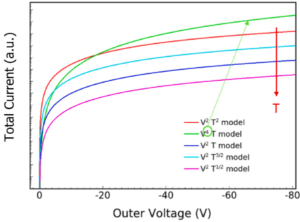
Fig. 7. Simulated I-V curves at different potential and temperature dependencies ( T=300\text{K} ).
