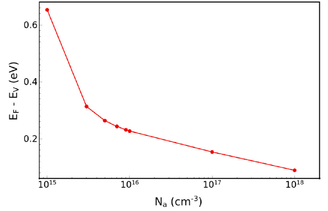
Fig. 4. Effect of the trapped charge concentration/effective doping concentration of the Fermi's level position. Arbitrarily high acceptor dopant concentrations have been considered.
