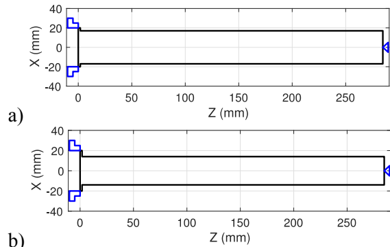
Fig. 9 Case B (overhang 287.5 mm) a) stock D: 28 mm b) final D: 24 mm.
