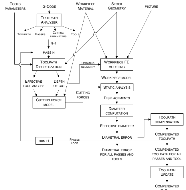
Fig. 2 General overview of the compensation algorithm.
