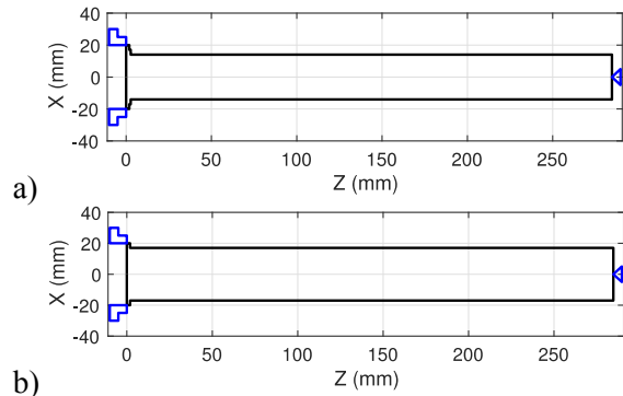
Fig. 8 Case A (overhang 287.5 mm) a) stock D: 34 mm b) final D: 28 mm.
