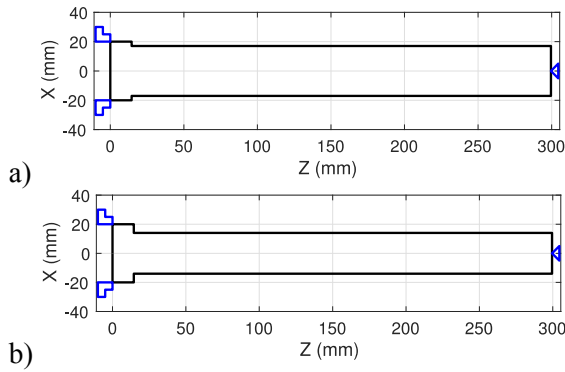
Fig. 10 Case C (overhang 299.5 mm) a) stock D: 34 mm b) final D: 28 mm.
